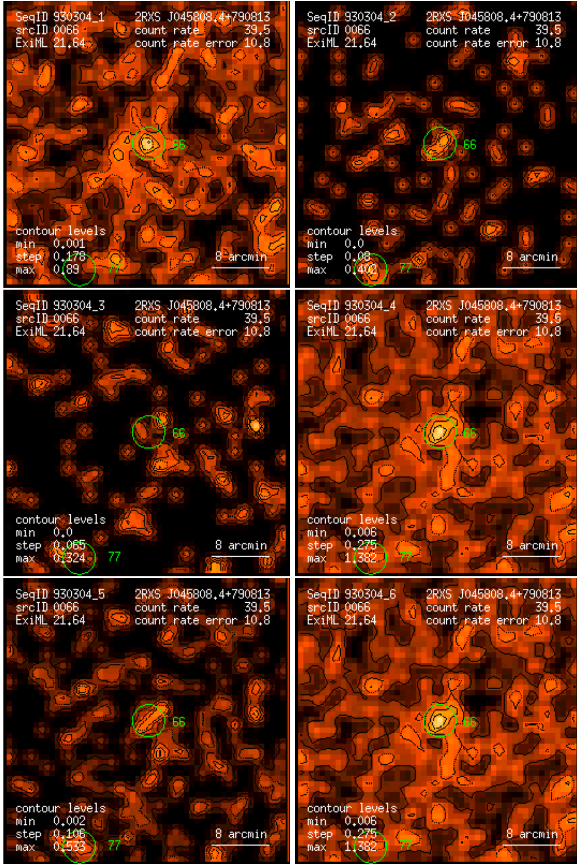
Figure 66: RASS 930304: detection 0066: band rate images, Gaussian filter: (1) PSPC channels 11 – 41, (2) 52 – 90, (3) 91 – 201, (4) 11 – 235, (5) 52 – 201, (6) 11 – 201. Broad band rates in counts/ks. Band rate contour levels in counts/ks/arcmin 2 .
