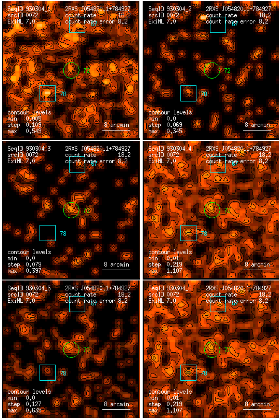
Figure 72: RASS 930304: detection 0072: band rate images, Gaussian filter: (1) PSPC channels 11 – 41, (2) 52 – 90, (3) 91 – 201, (4) 11 – 235, (5) 52 – 201, (6) 11 – 201. Broad band rates in counts/ks. Band rate contour levels in counts/ks/arcmin 2 .
