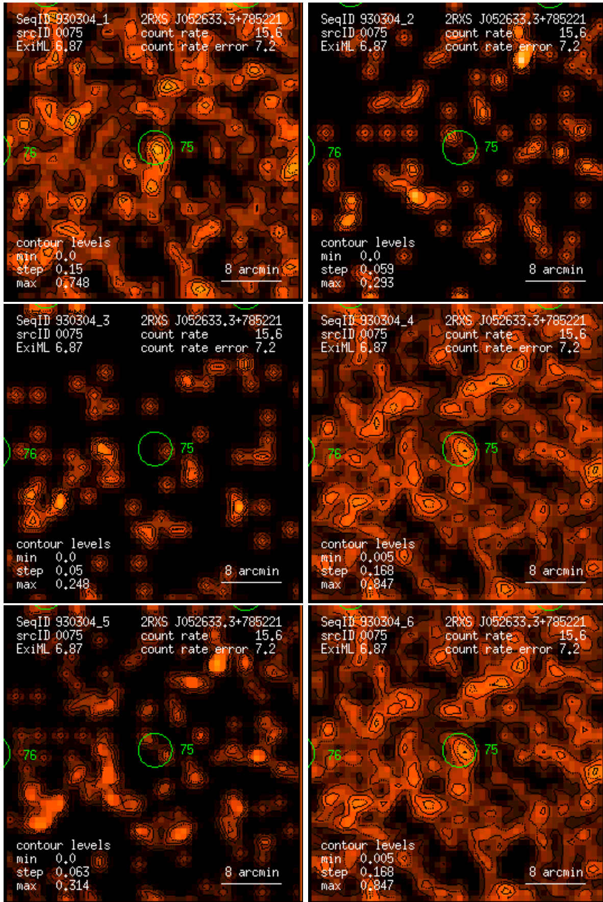
Figure 75: RASS 930304: detection 0075: band rate images, Gaussian filter: (1) PSPC channels 11 – 41, (2) 52 – 90, (3) 91 – 201, (4) 11 – 235, (5) 52 – 201, (6) 11 – 201. Broad band rates in counts/ks. Band rate contour levels in counts/ks/arcmin 2 .
