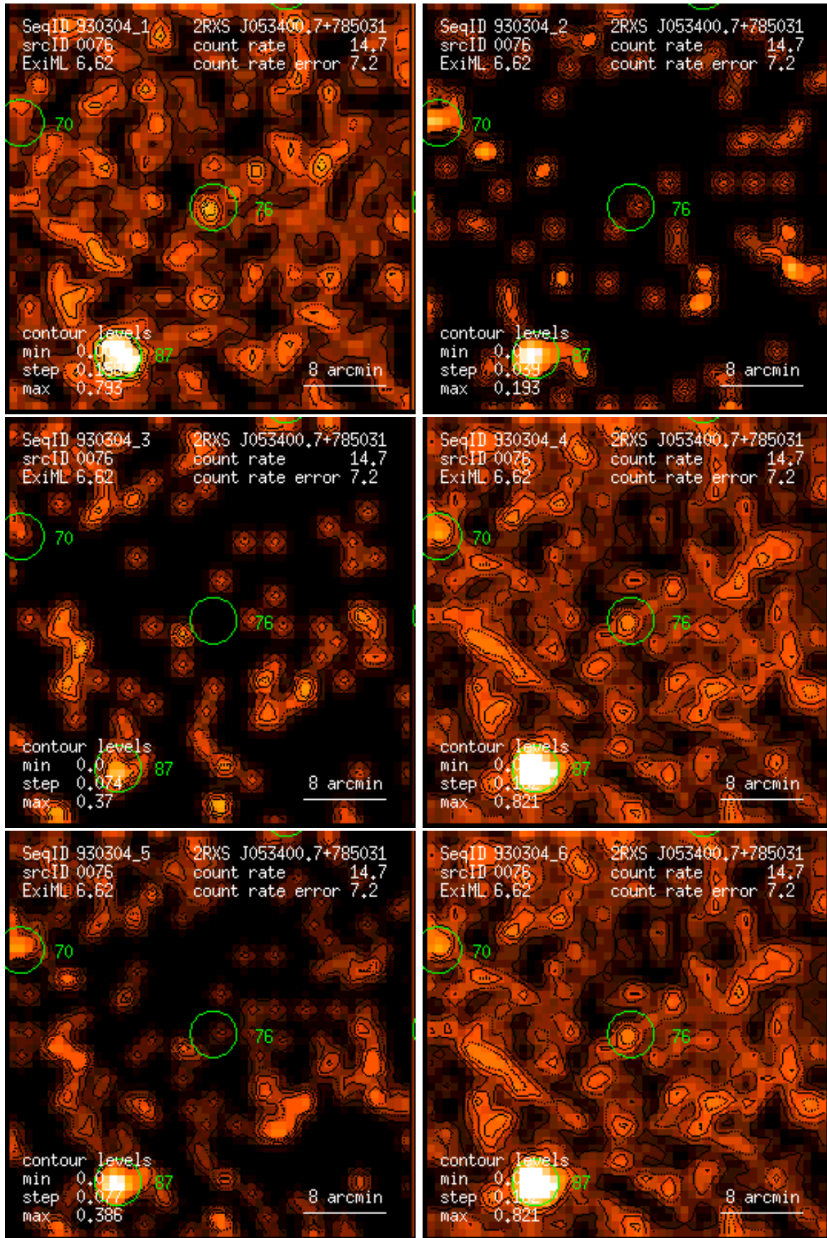
Figure 76: RASS 930304: detection 0076: band rate images, Gaussian filter: (1) PSPC channels 11 – 41, (2) 52 – 90, (3) 91 – 201, (4) 11 – 235, (5) 52 – 201, (6) 11 – 201. Broad band rates in counts/ks. Band rate contour levels in counts/ks/arcmin 2 .
