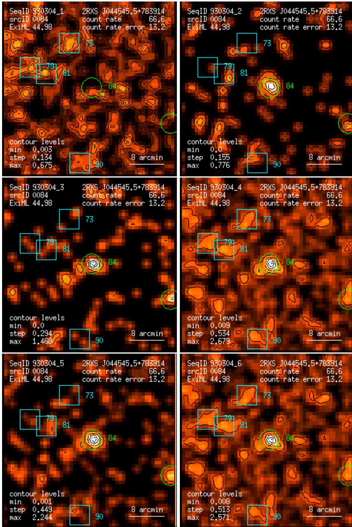
Figure 84: RASS 930304: detection 0084: band rate images, Gaussian filter: (1) PSPC channels 11 – 41, (2) 52 – 90, (3) 91 – 201, (4) 11 – 235, (5) 52 – 201, (6) 11 – 201. Broad band rates in counts/ks. Band rate contour levels in counts/ks/arcmin 2 .
