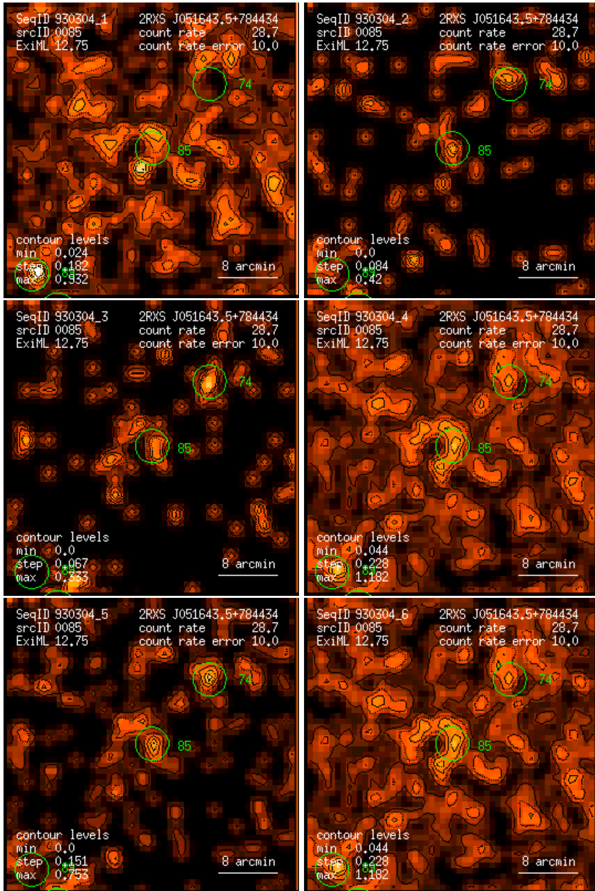
Figure 85: RASS 930304: detection 0085: band rate images, Gaussian filter: (1) PSPC channels 11 – 41, (2) 52 – 90, (3) 91 – 201, (4) 11 – 235, (5) 52 – 201, (6) 11 – 201. Broad band rates in counts/ks. Band rate contour levels in counts/ks/arcmin 2 .
