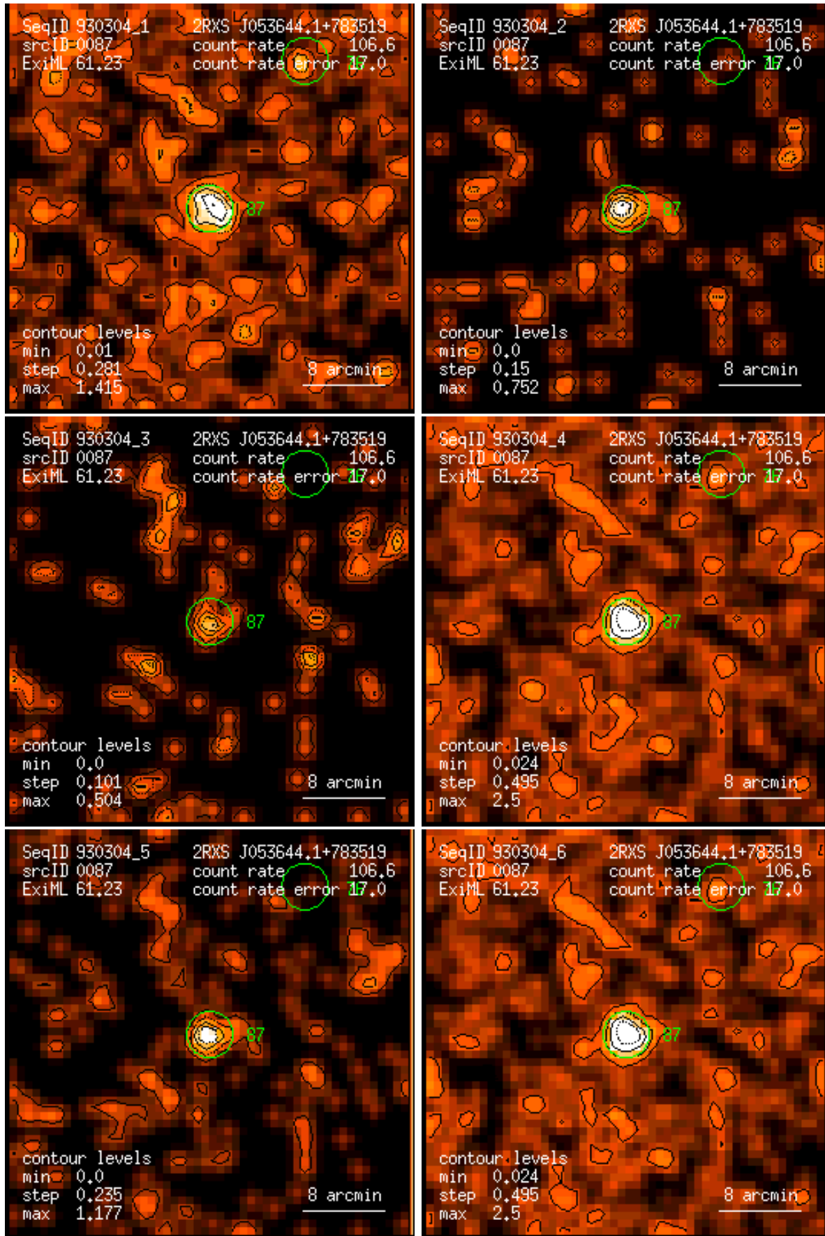
Figure 87: RASS 930304: detection 0087: band rate images, Gaussian filter: (1) PSPC channels 11 – 41, (2) 52 – 90, (3) 91 – 201, (4) 11 – 235, (5) 52 – 201, (6) 11 – 201. Broad band rates in counts/ks. Band rate contour levels in counts/ks/arcmin 2 .
