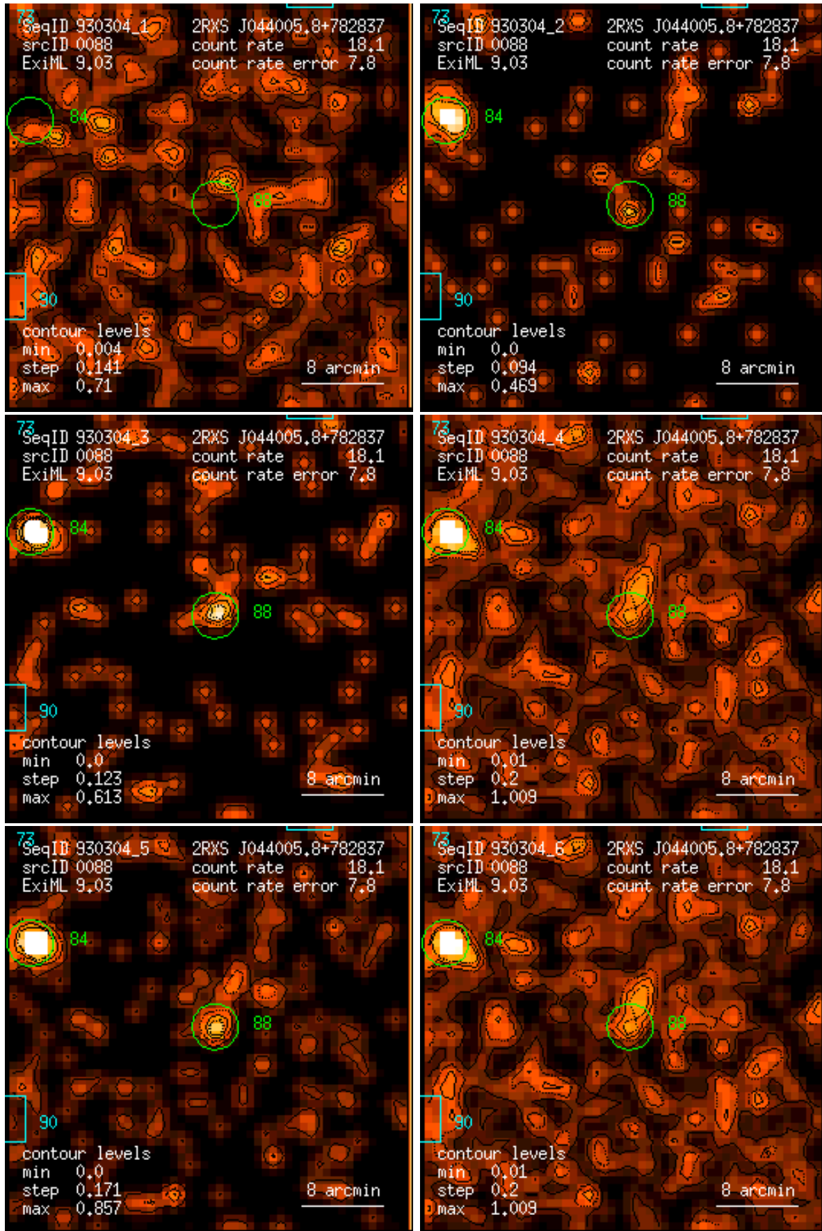
Figure 88: RASS 930304: detection 0088: band rate images, Gaussian filter: (1) PSPC channels 11 – 41, (2) 52 – 90, (3) 91 – 201, (4) 11 – 235, (5) 52 – 201, (6) 11 – 201. Broad band rates in counts/ks. Band rate contour levels in counts/ks/arcmin 2 .
