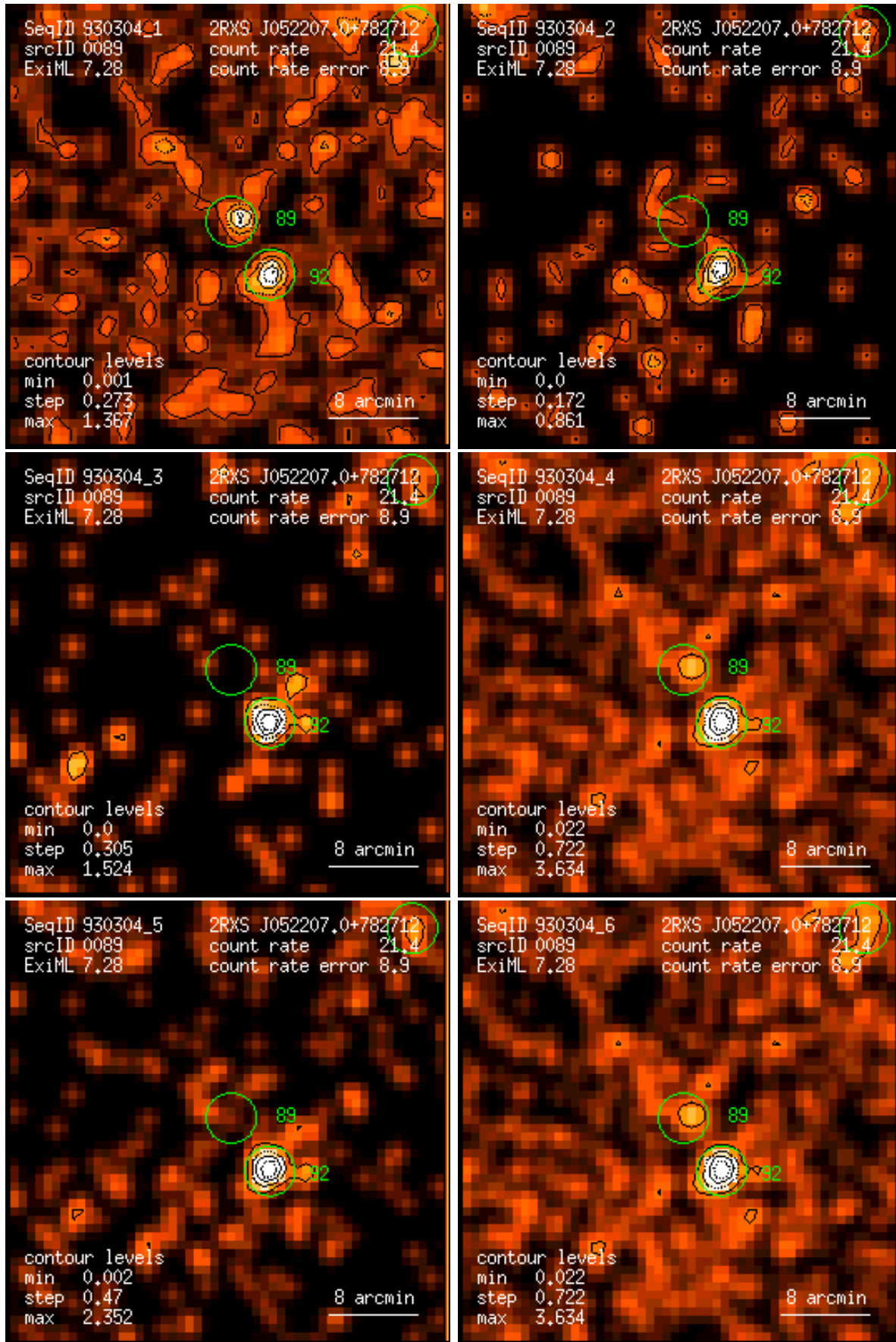
Figure 89: RASS 930304: detection 0089: band rate images, Gaussian filter: (1) PSPC channels 11 – 41, (2) 52 – 90, (3) 91 – 201, (4) 11 – 235, (5) 52 – 201, (6) 11 – 201. Broad band rates in counts/ks. Band rate contour levels in counts/ks/arcmin 2 .
