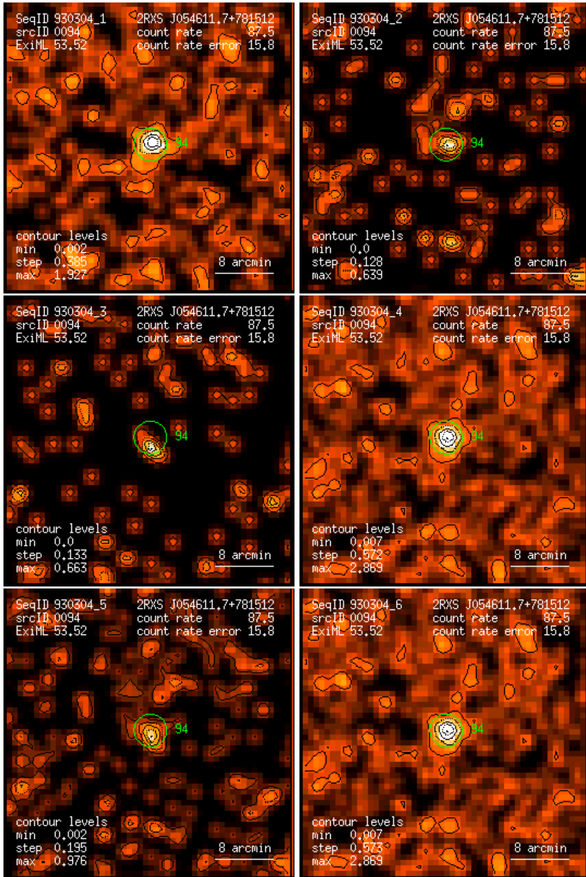
Figure 94: RASS 930304: detection 0094: band rate images, Gaussian filter: (1) PSPC channels 11 – 41, (2) 52 – 90, (3) 91 – 201, (4) 11 – 235, (5) 52 – 201, (6) 11 – 201. Broad band rates in counts/ks. Band rate contour levels in counts/ks/arcmin 2 .
