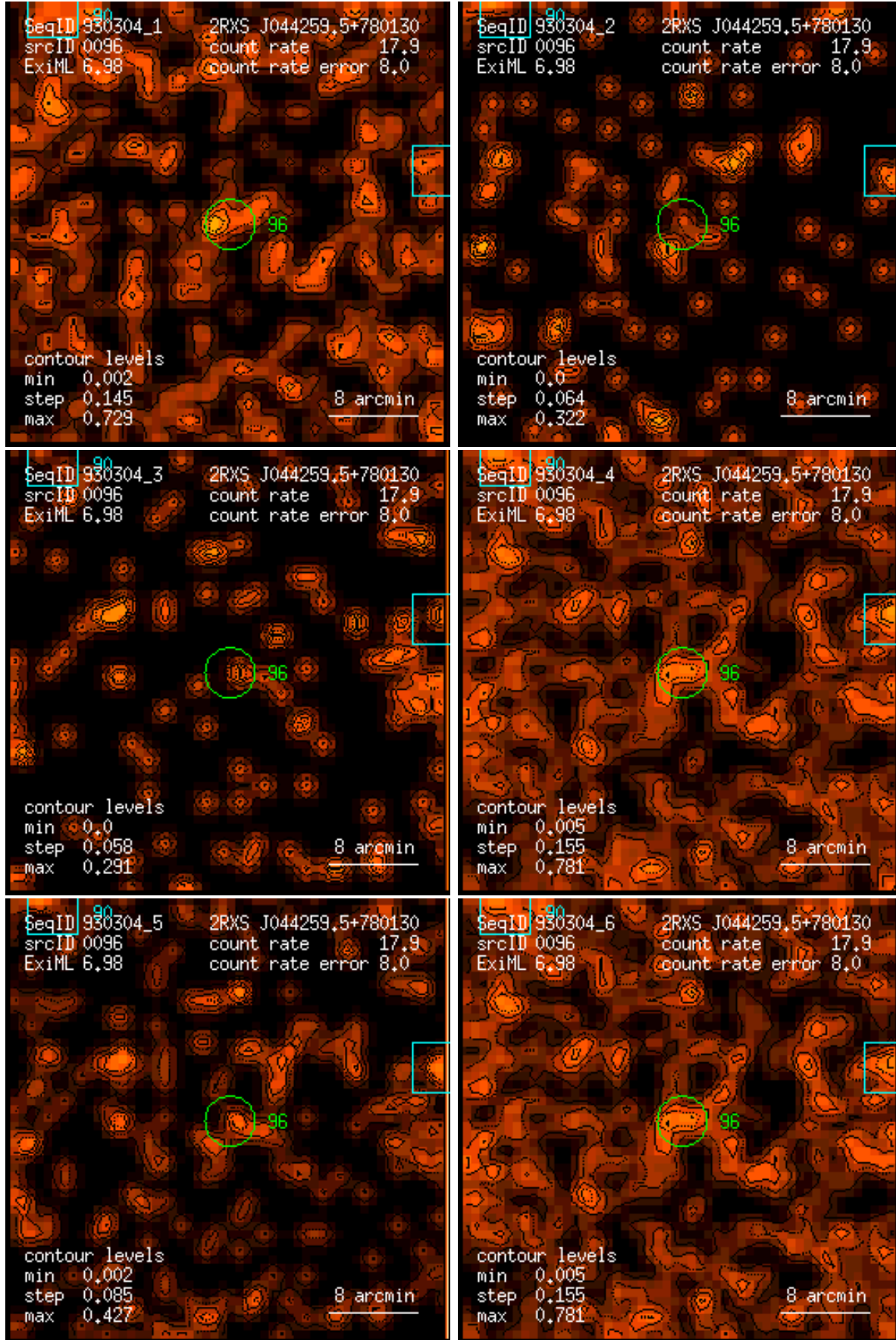
Figure 96: RASS 930304: detection 0096: band rate images, Gaussian filter: (1) PSPC channels 11 – 41, (2) 52 – 90, (3) 91 – 201, (4) 11 – 235, (5) 52 – 201, (6) 11 – 201. Broad band rates in counts/ks. Band rate contour levels in counts/ks/arcmin 2 .
