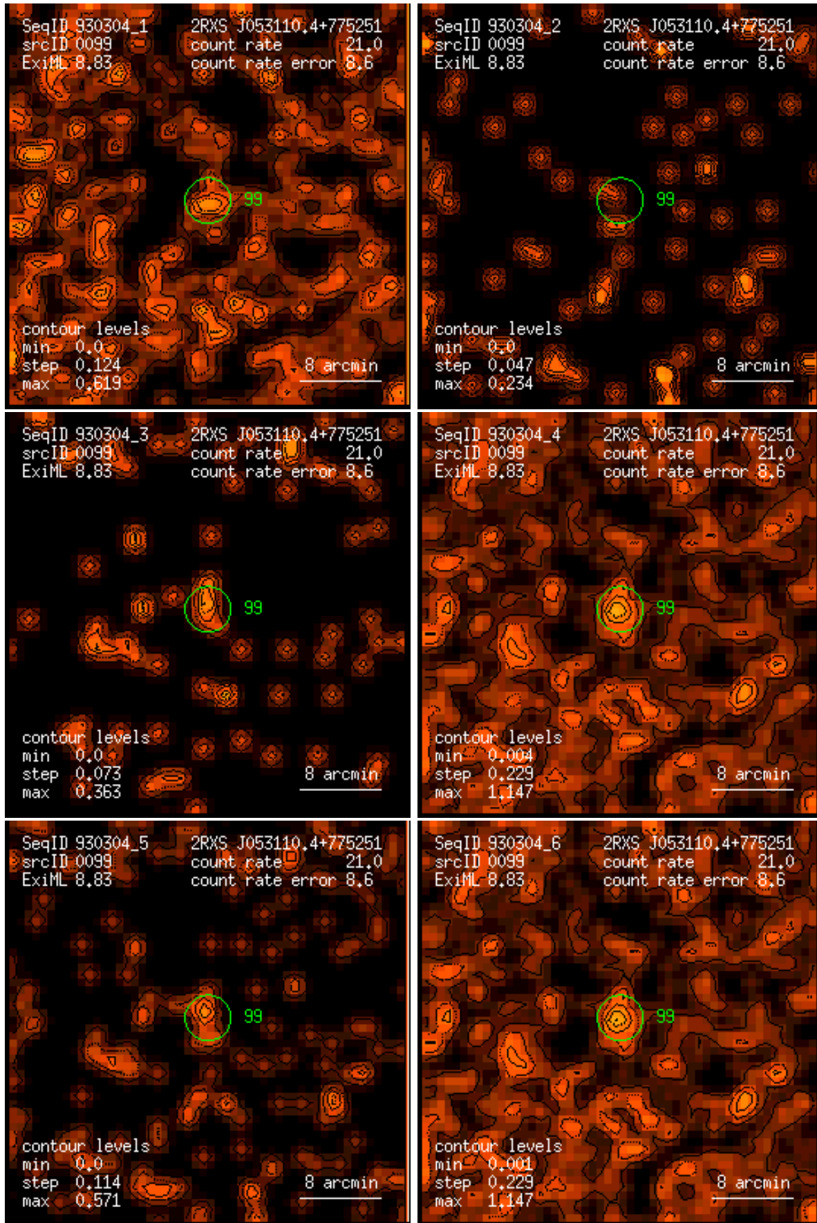
Figure 99: RASS 930304: detection 0099: band rate images, Gaussian filter: (1) PSPC channels 11 – 41, (2) 52 – 90, (3) 91 – 201, (4) 11 – 235, (5) 52 – 201, (6) 11 – 201. Broad band rates in counts/ks. Band rate contour levels in counts/ks/arcmin 2 .
