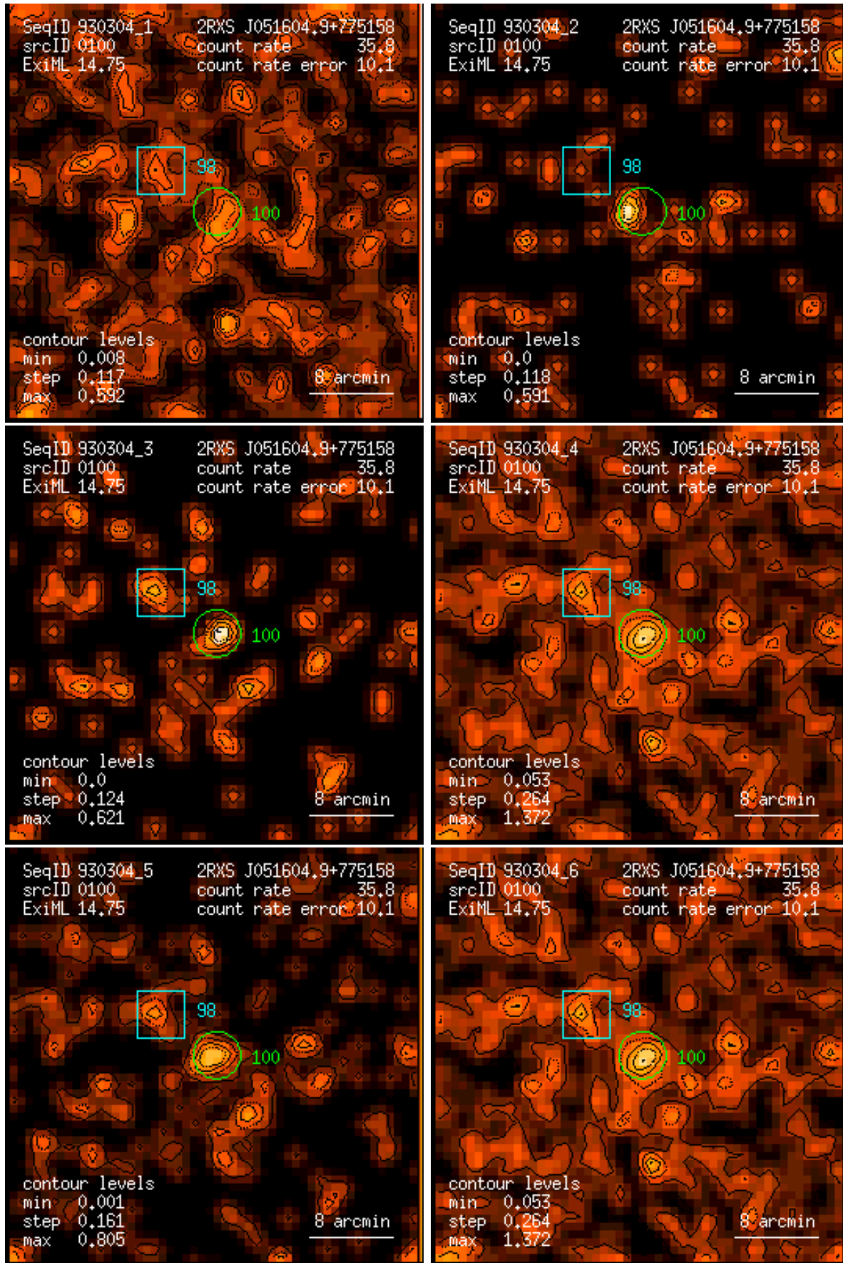
Figure 100: RASS 930304: detection 0100: band rate images, Gaussian filter: (1) PSPC channels 11 – 41, (2) 52 – 90, (3) 91 – 201, (4) 11 – 235, (5) 52 – 201, (6) 11 – 201. Broad band rates in counts/ks. Band rate contour levels in counts/ks/arcmin 2 .
