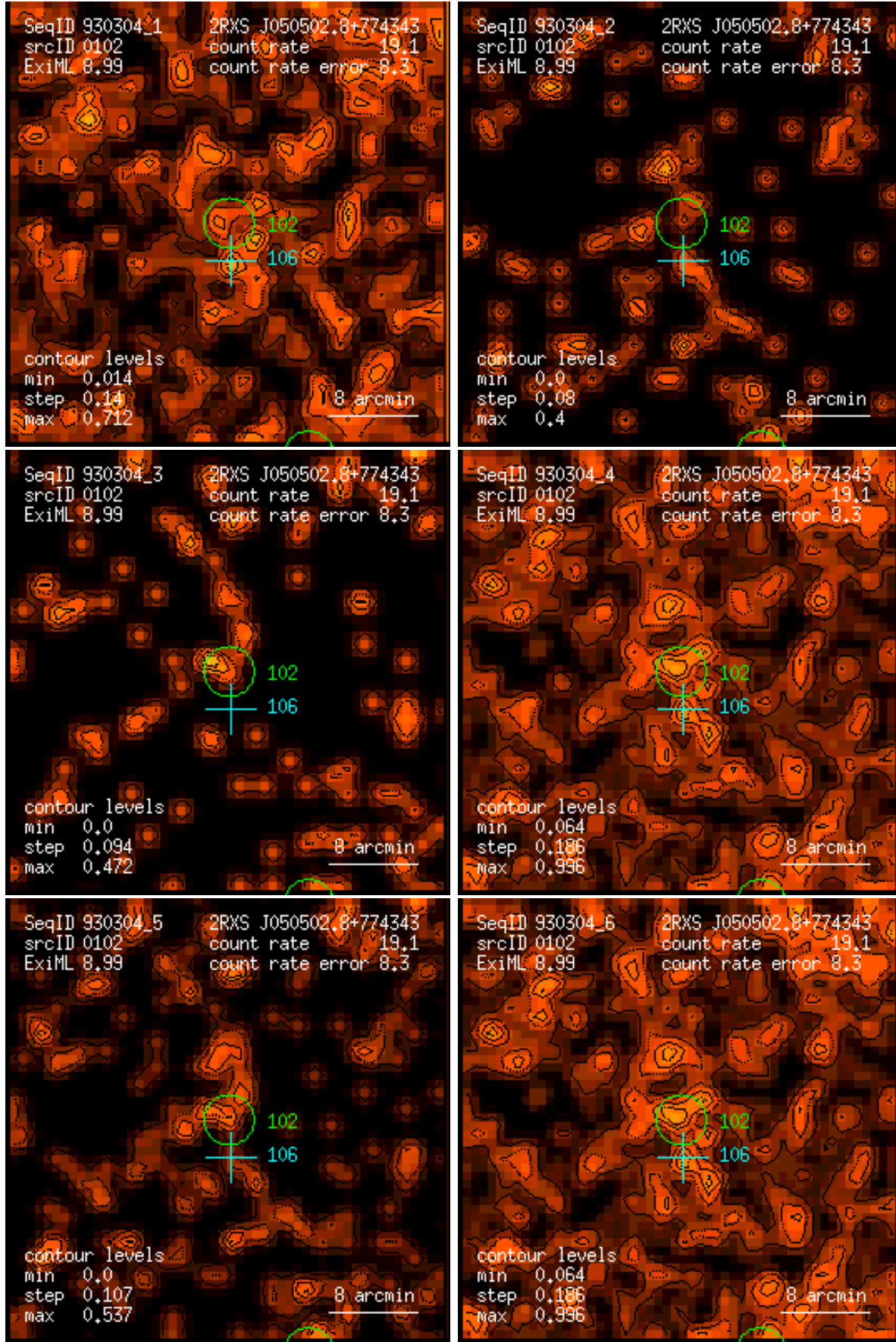
Figure 102: RASS 930304: detection 0102: band rate images, Gaussian filter: (1) PSPC channels 11 – 41, (2) 52 – 90, (3) 91 – 201, (4) 11 – 235, (5) 52 – 201, (6) 11 – 201. Broad band rates in counts/ks. Band rate contour levels in counts/ks/arcmin 2 .
