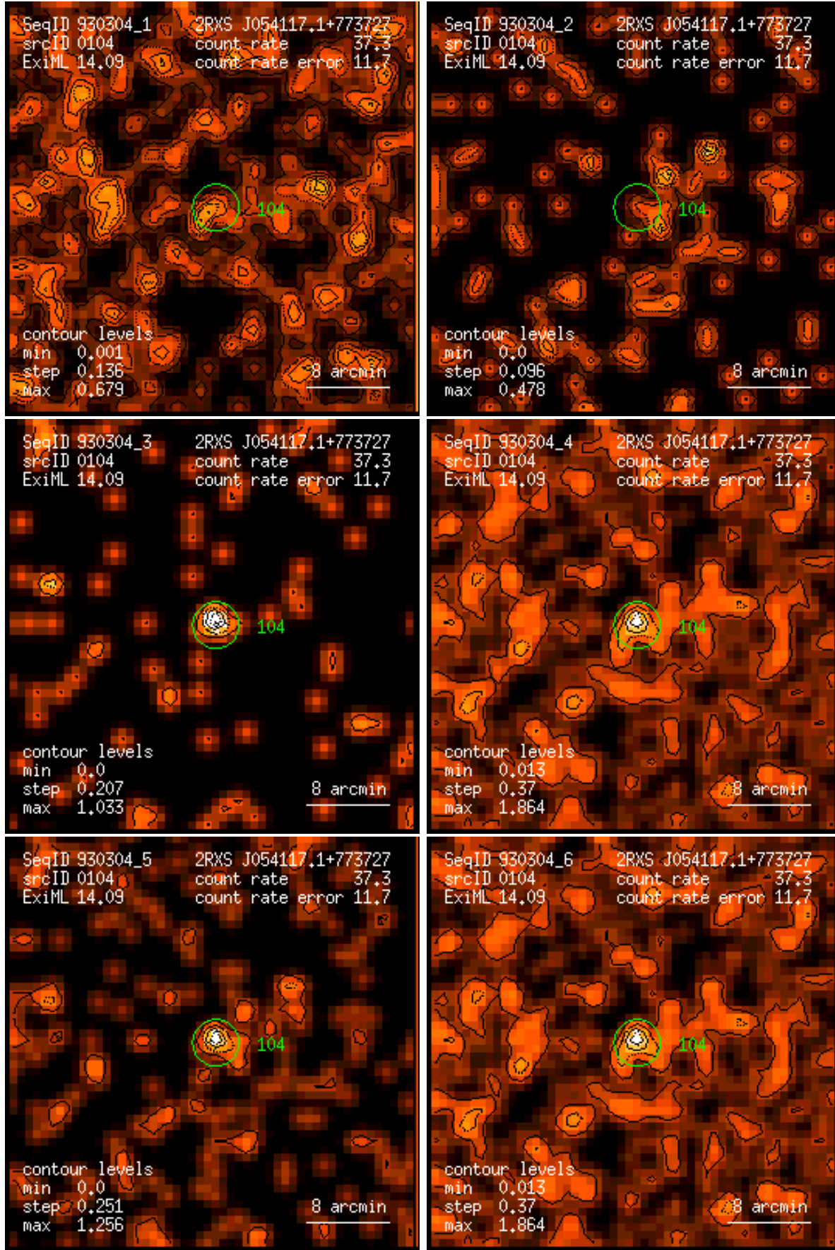
Figure 104: RASS 930304: detection 0104: band rate images, Gaussian filter: (1) PSPC channels 11 – 41, (2) 52 – 90, (3) 91 – 201, (4) 11 – 235, (5) 52 – 201, (6) 11 – 201. Broad band rates in counts/ks. Band rate contour levels in counts/ks/arcmin 2 .
