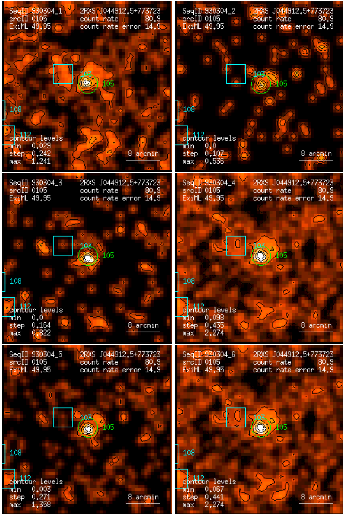
Figure 105: RASS 930304: detection 0105: band rate images, Gaussian filter: (1) PSPC channels 11 – 41, (2) 52 – 90, (3) 91 – 201, (4) 11 – 235, (5) 52 – 201, (6) 11 – 201. Broad band rates in counts/ks. Band rate contour levels in counts/ks/arcmin 2 .
