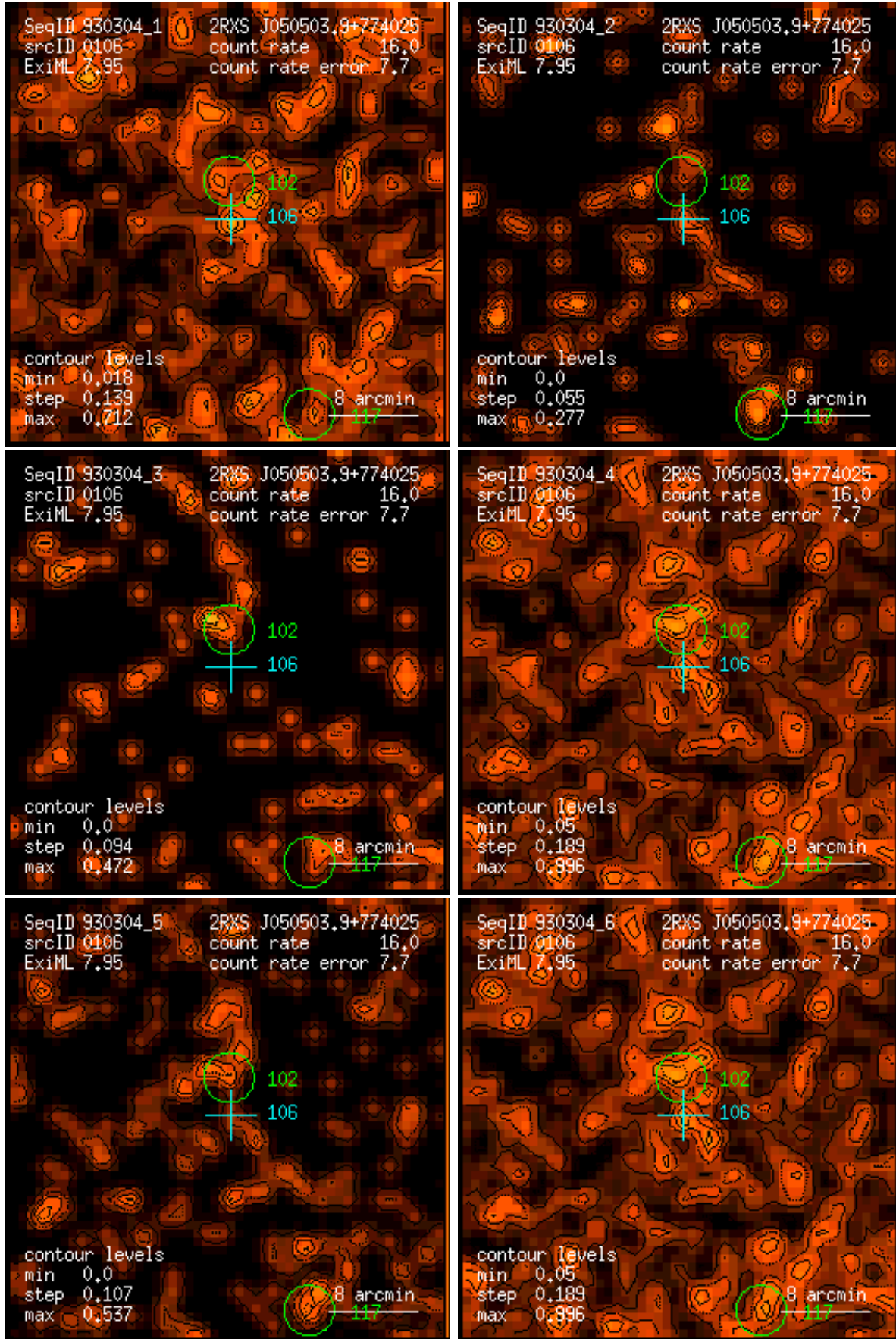
Figure 106: RASS 930304: detection 0106: band rate images, Gaussian filter: (1) PSPC channels 11 – 41, (2) 52 – 90, (3) 91 – 201, (4) 11 – 235, (5) 52 – 201, (6) 11 – 201. Broad band rates in counts/ks. Band rate contour levels in counts/ks/arcmin 2 .
