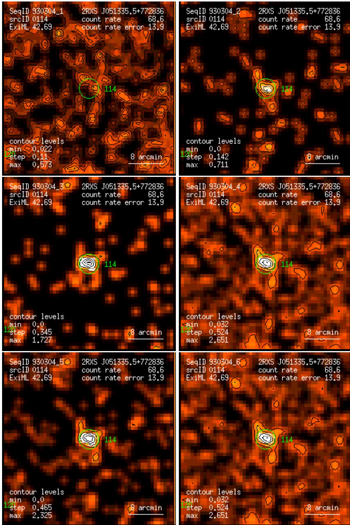
Figure 114: RASS 930304: detection 0114: band rate images, Gaussian filter: (1) PSPC channels 11 – 41, (2) 52 – 90, (3) 91 – 201, (4) 11 – 235, (5) 52 – 201, (6) 11 – 201. Broad band rates in counts/ks. Band rate contour levels in counts/ks/arcmin 2 .
