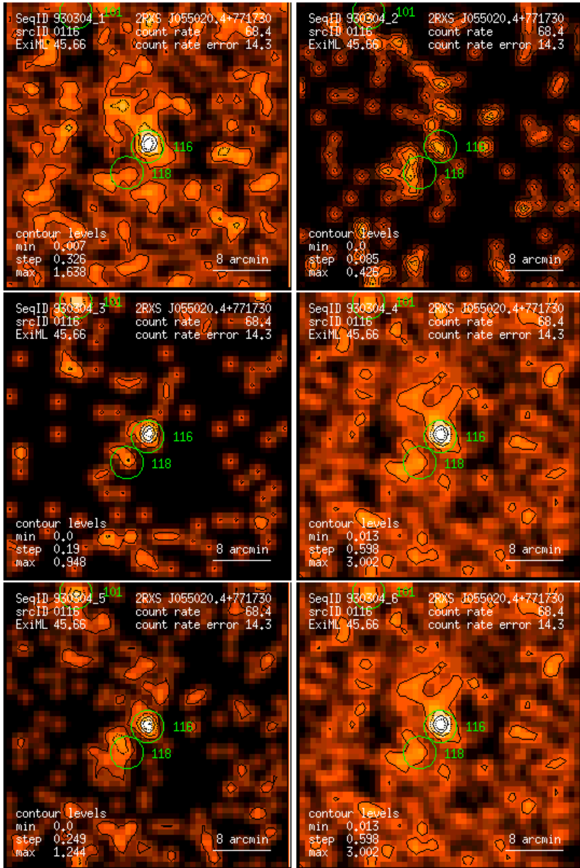
Figure 116: RASS 930304: detection 0116: band rate images, Gaussian filter: (1) PSPC channels 11 – 41, (2) 52 – 90, (3) 91 – 201, (4) 11 – 235, (5) 52 – 201, (6) 11 – 201. Broad band rates in counts/ks. Band rate contour levels in counts/ks/arcmin 2 .
