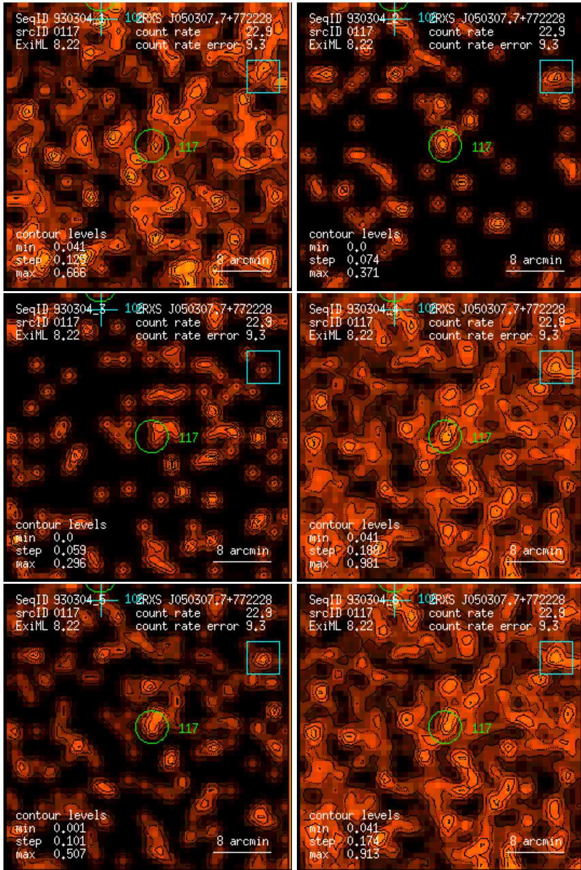
Figure 117: RASS 930304: detection 0117: band rate images, Gaussian filter: (1) PSPC channels 11 – 41, (2) 52 – 90, (3) 91 – 201, (4) 11 – 235, (5) 52 – 201, (6) 11 – 201. Broad band rates in counts/ks. Band rate contour levels in counts/ks/arcmin 2 .
