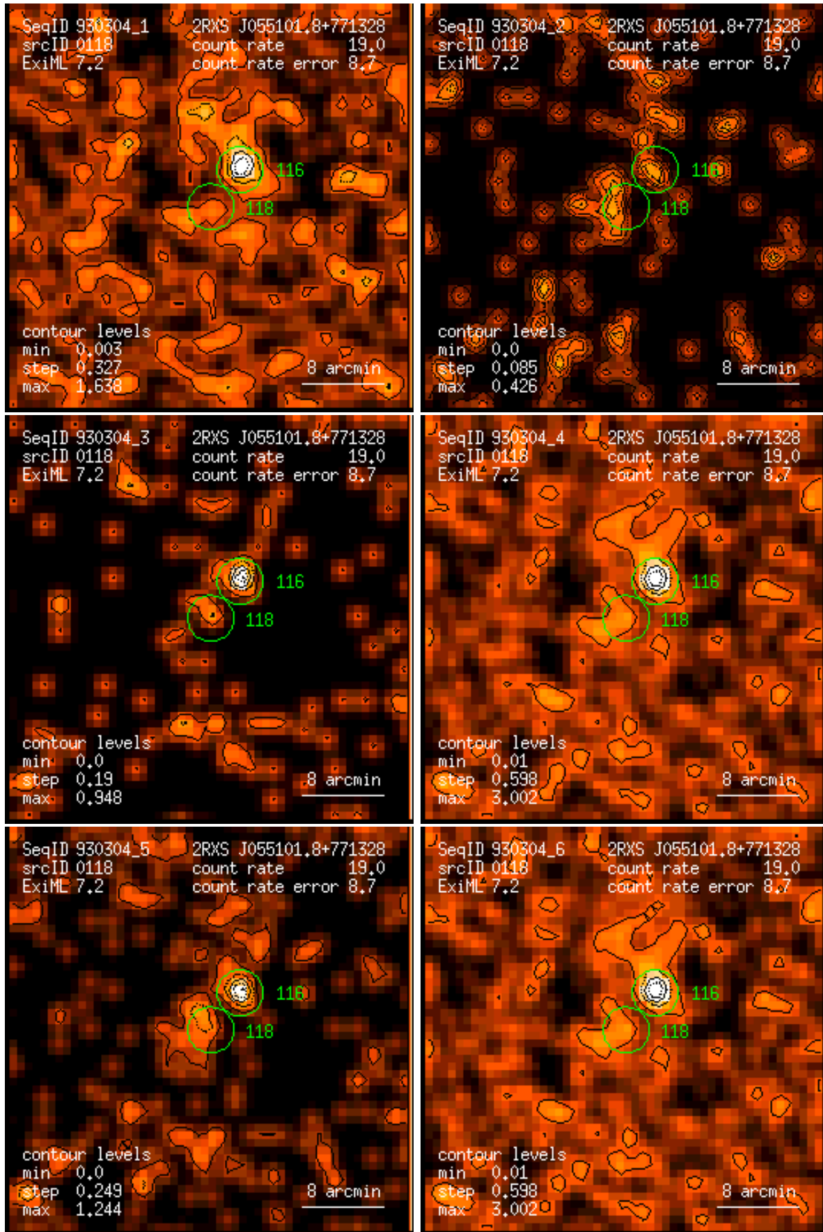
Figure 118: RASS 930304: detection 0118: band rate images, Gaussian filter: (1) PSPC channels 11 – 41, (2) 52 – 90, (3) 91 – 201, (4) 11 – 235, (5) 52 – 201, (6) 11 – 201. Broad band rates in counts/ks. Band rate contour levels in counts/ks/arcmin 2 .
