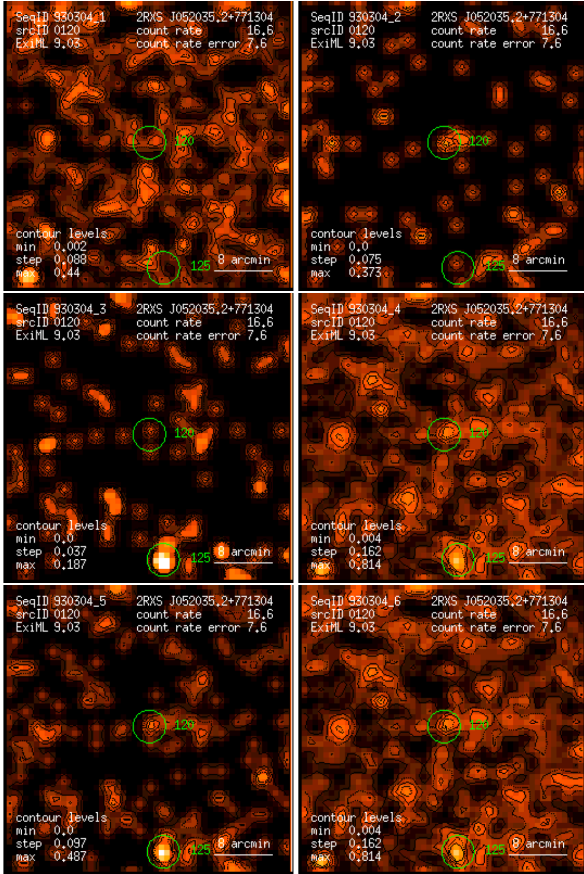
Figure 120: RASS 930304: detection 0120: band rate images, Gaussian filter: (1) PSPC channels 11 – 41, (2) 52 – 90, (3) 91 – 201, (4) 11 – 235, (5) 52 – 201, (6) 11 – 201. Broad band rates in counts/ks. Band rate contour levels in counts/ks/arcmin 2 .
