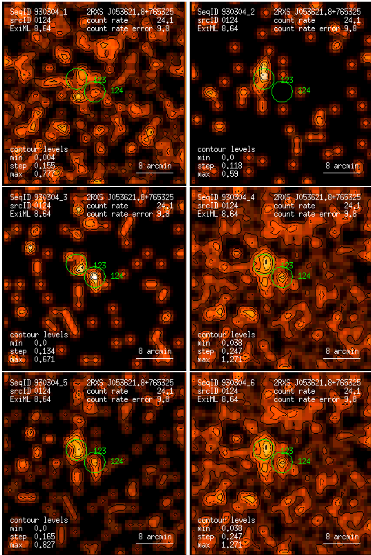
Figure 124: RASS 930304: detection 0124: band rate images, Gaussian filter: (1) PSPC channels 11 – 41, (2) 52 – 90, (3) 91 – 201, (4) 11 – 235, (5) 52 – 201, (6) 11 – 201. Broad band rates in counts/ks. Band rate contour levels in counts/ks/arcmin 2 .
