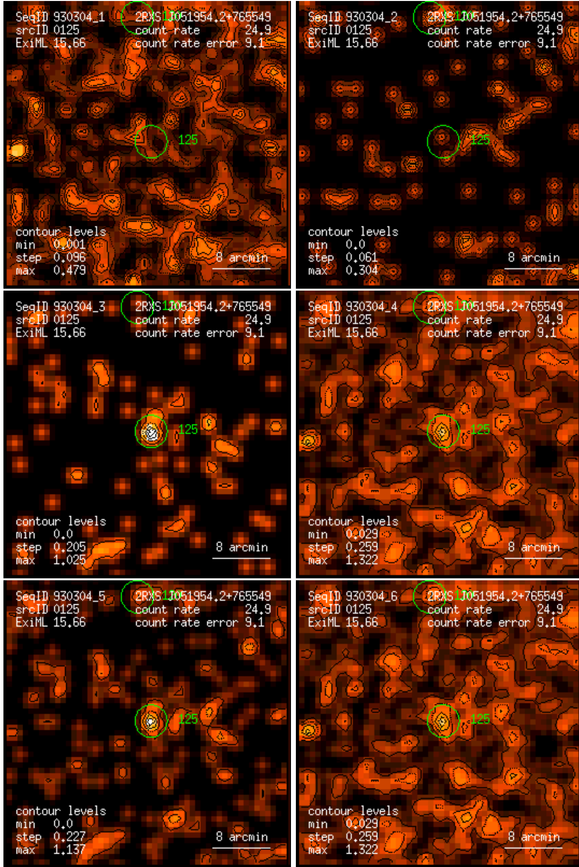
Figure 125: RASS 930304: detection 0125: band rate images, Gaussian filter: (1) PSPC channels 11 – 41, (2) 52 – 90, (3) 91 – 201, (4) 11 – 235, (5) 52 – 201, (6) 11 – 201. Broad band rates in counts/ks. Band rate contour levels in counts/ks/arcmin 2 .
