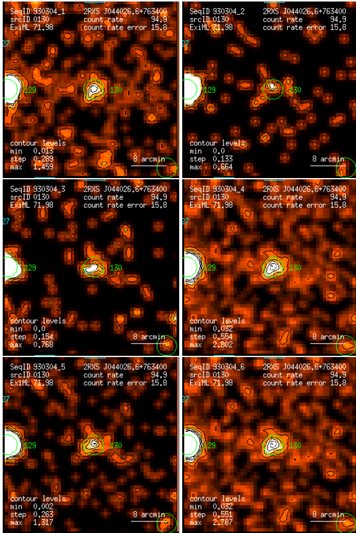
Figure 130: RASS 930304: detection 0130: band rate images, Gaussian filter: (1) PSPC channels 11 – 41, (2) 52 – 90, (3) 91 – 201, (4) 11 – 235, (5) 52 – 201, (6) 11 – 201. Broad band rates in counts/ks. Band rate contour levels in counts/ks/arcmin 2 .
