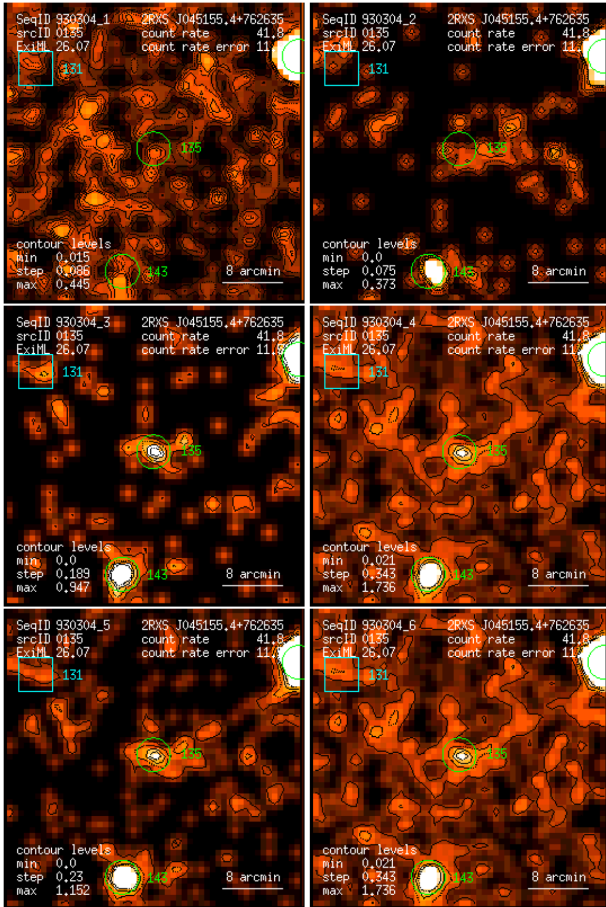
Figure 135: RASS 930304: detection 0135: band rate images, Gaussian filter: (1) PSPC channels 11 – 41, (2) 52 – 90, (3) 91 – 201, (4) 11 – 235, (5) 52 – 201, (6) 11 – 201. Broad band rates in counts/ks. Band rate contour levels in counts/ks/arcmin 2 .
