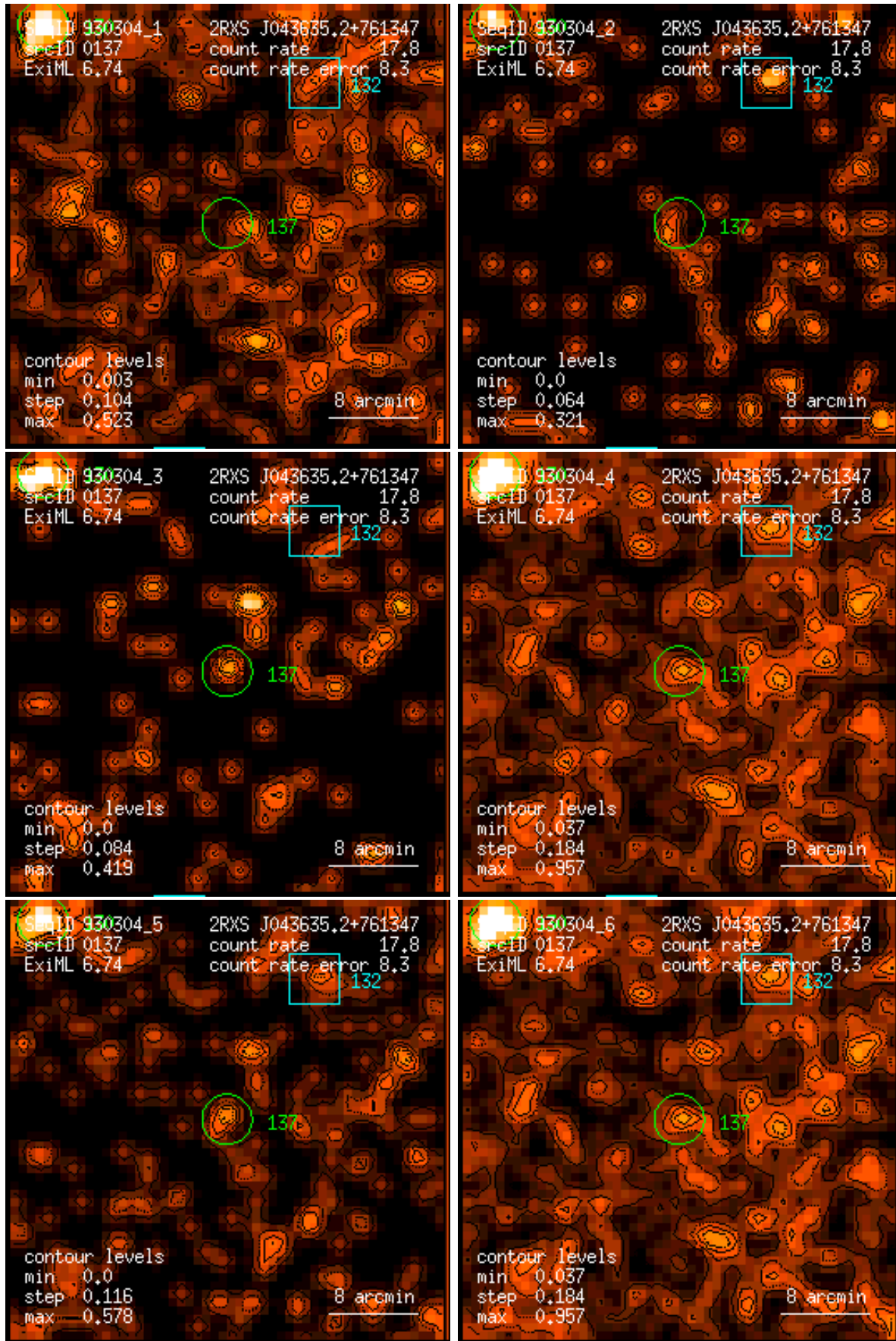
Figure 137: RASS 930304: detection 0137: band rate images, Gaussian filter: (1) PSPC channels 11 – 41, (2) 52 – 90, (3) 91 – 201, (4) 11 – 235, (5) 52 – 201, (6) 11 – 201. Broad band rates in counts/ks. Band rate contour levels in counts/ks/arcmin 2 .
