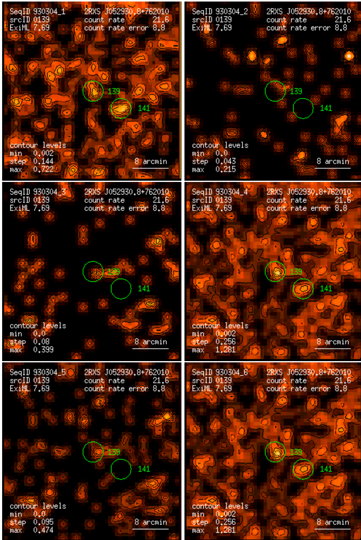
Figure 139: RASS 930304: detection 0139: band rate images, Gaussian filter: (1) PSPC channels 11 – 41, (2) 52 – 90, (3) 91 – 201, (4) 11 – 235, (5) 52 – 201, (6) 11 – 201. Broad band rates in counts/ks. Band rate contour levels in counts/ks/arcmin 2 .
