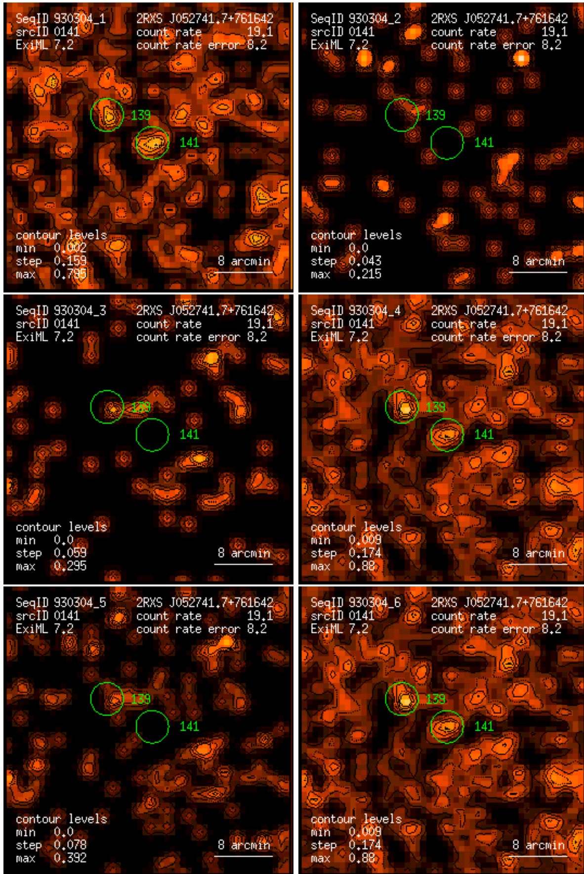
Figure 141: RASS 930304: detection 0141: band rate images, Gaussian filter: (1) PSPC channels 11 – 41, (2) 52 – 90, (3) 91 – 201, (4) 11 – 235, (5) 52 – 201, (6) 11 – 201. Broad band rates in counts/ks. Band rate contour levels in counts/ks/arcmin 2 .
