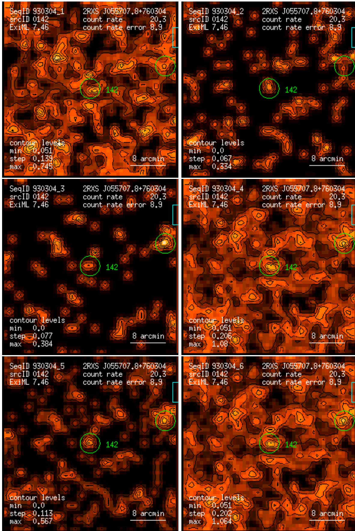
Figure 142: RASS 930304: detection 0142: band rate images, Gaussian filter: (1) PSPC channels 11 – 41, (2) 52 – 90, (3) 91 – 201, (4) 11 – 235, (5) 52 – 201, (6) 11 – 201. Broad band rates in counts/ks. Band rate contour levels in counts/ks/arcmin 2 .
