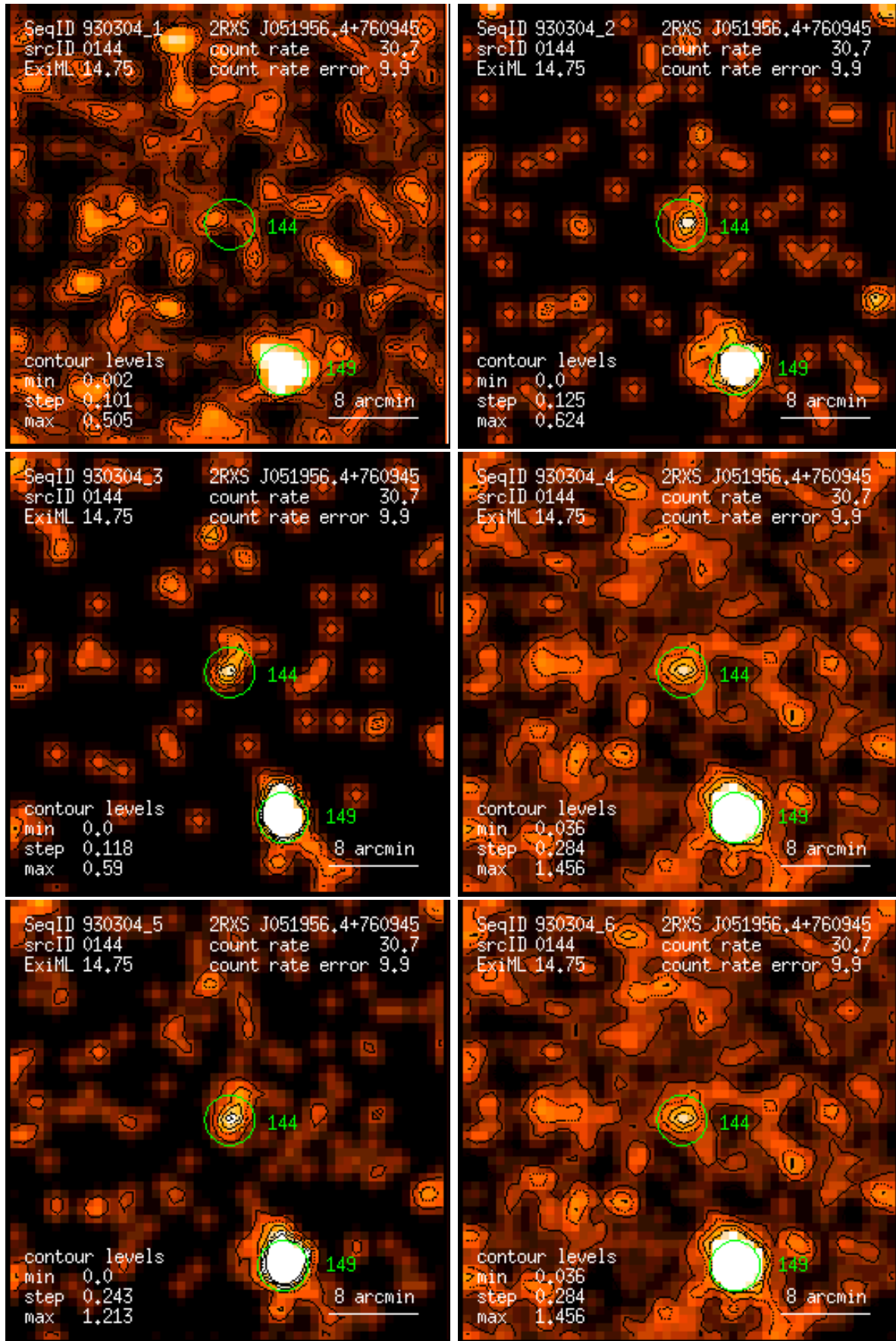
Figure 144: RASS 930304: detection 0144: band rate images, Gaussian filter: (1) PSPC channels 11 – 41, (2) 52 – 90, (3) 91 – 201, (4) 11 – 235, (5) 52 – 201, (6) 11 – 201. Broad band rates in counts/ks. Band rate contour levels in counts/ks/arcmin 2 .
