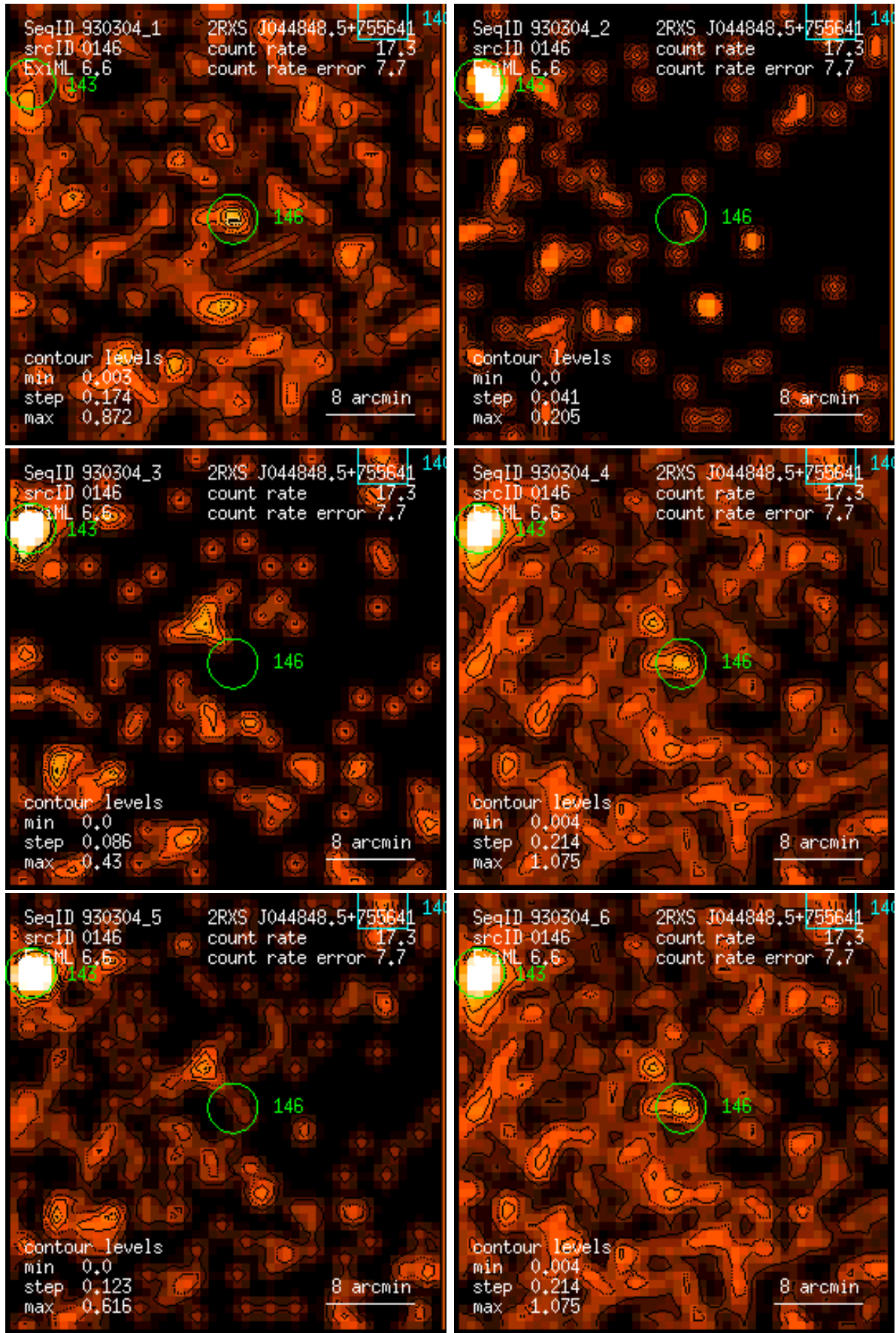
Figure 146: RASS 930304: detection 0146: band rate images, Gaussian filter: (1) PSPC channels 11 – 41, (2) 52 – 90, (3) 91 – 201, (4) 11 – 235, (5) 52 – 201, (6) 11 – 201. Broad band rates in counts/ks. Band rate contour levels in counts/ks/arcmin 2 .
