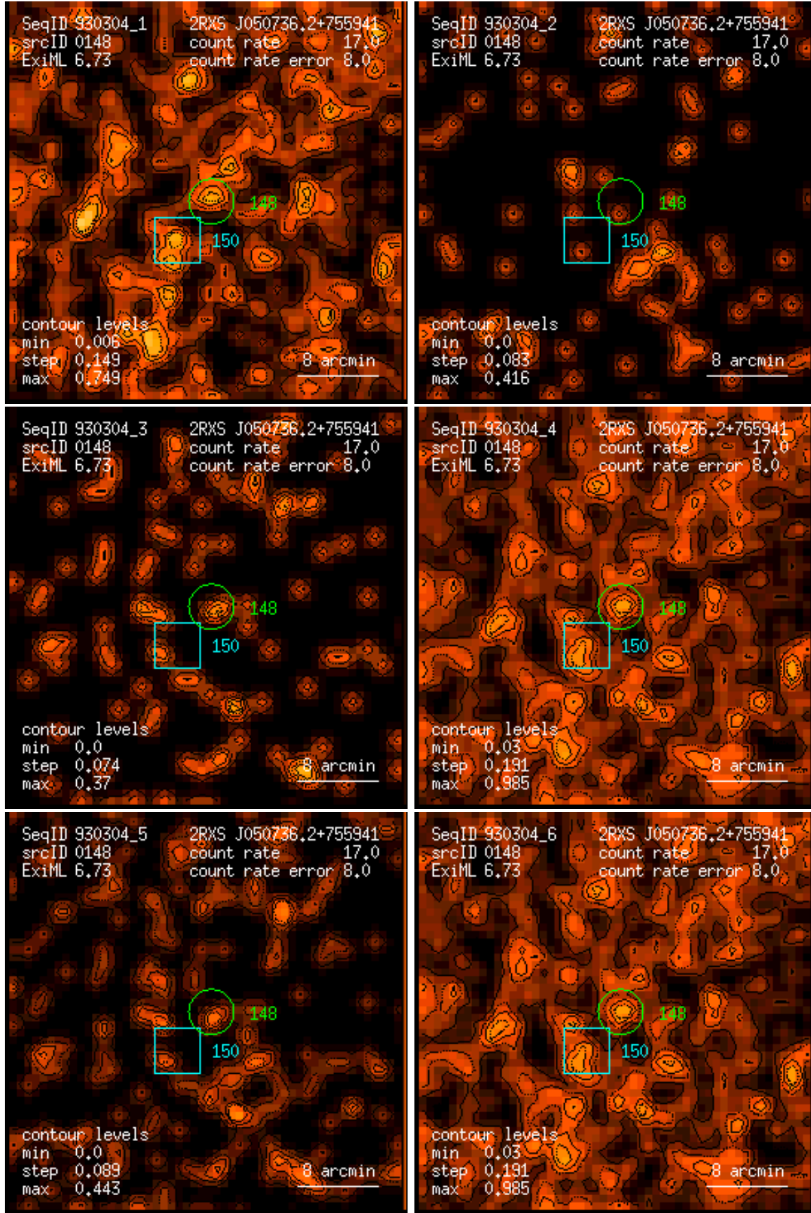
Figure 148: RASS 930304: detection 0148: band rate images, Gaussian filter: (1) PSPC channels 11 – 41, (2) 52 – 90, (3) 91 – 201, (4) 11 – 235, (5) 52 – 201, (6) 11 – 201. Broad band rates in counts/ks. Band rate contour levels in counts/ks/arcmin 2 .
