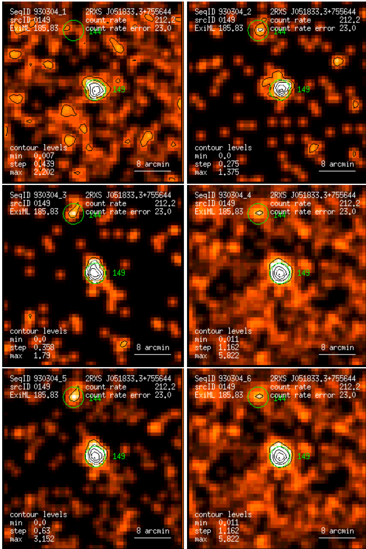
Figure 149: RASS 930304: detection 0149: band rate images, Gaussian filter: (1) PSPC channels 11 – 41, (2) 52 – 90, (3) 91 – 201, (4) 11 – 235, (5) 52 – 201, (6) 11 – 201. Broad band rates in counts/ks. Band rate contour levels in counts/ks/arcmin 2 .
