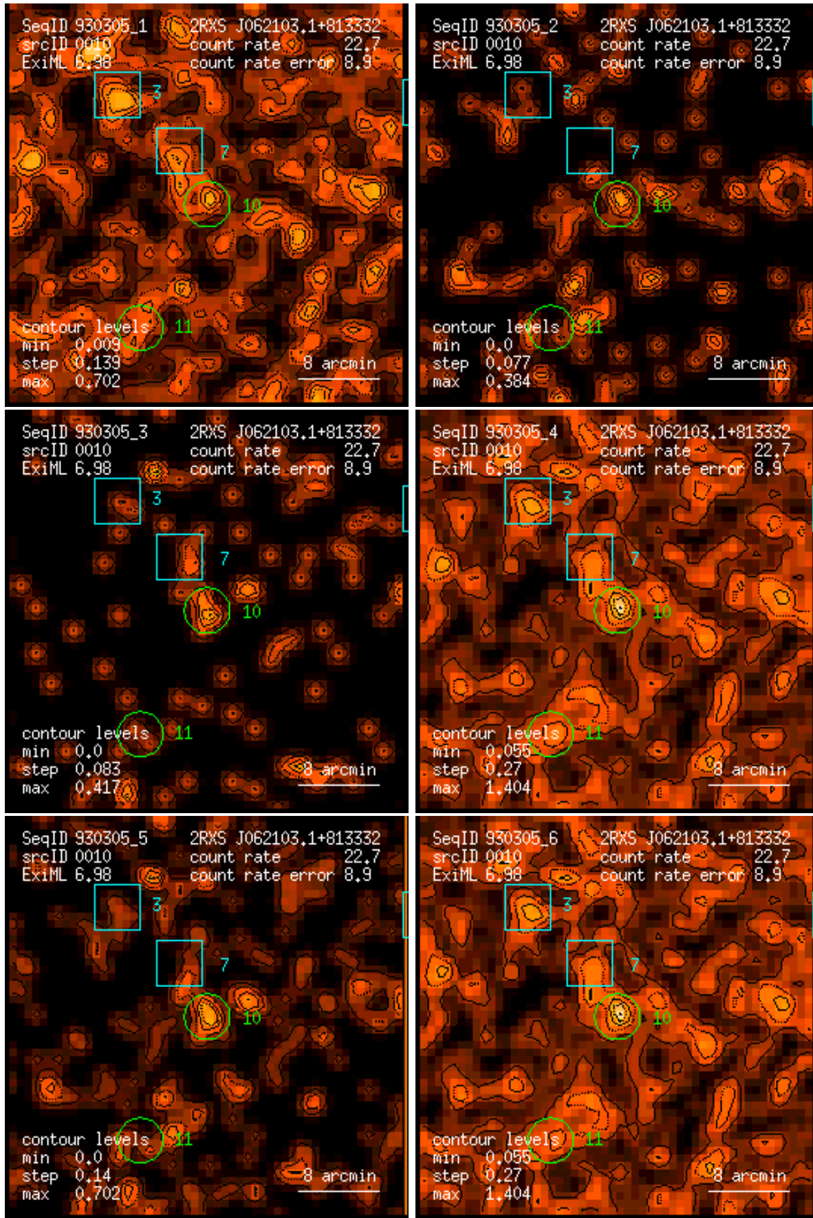
Figure 10: RASS 930305: detection 0010: band rate images, Gaussian filter: (1) PSPC channels 11 – 41, (2) 52 – 90, (3) 91 – 201, (4) 11 – 235, (5) 52 – 201, (6) 11 – 201. Broad band rates in counts/ks. Band rate contour levels in counts/ks/arcmin 2 .
