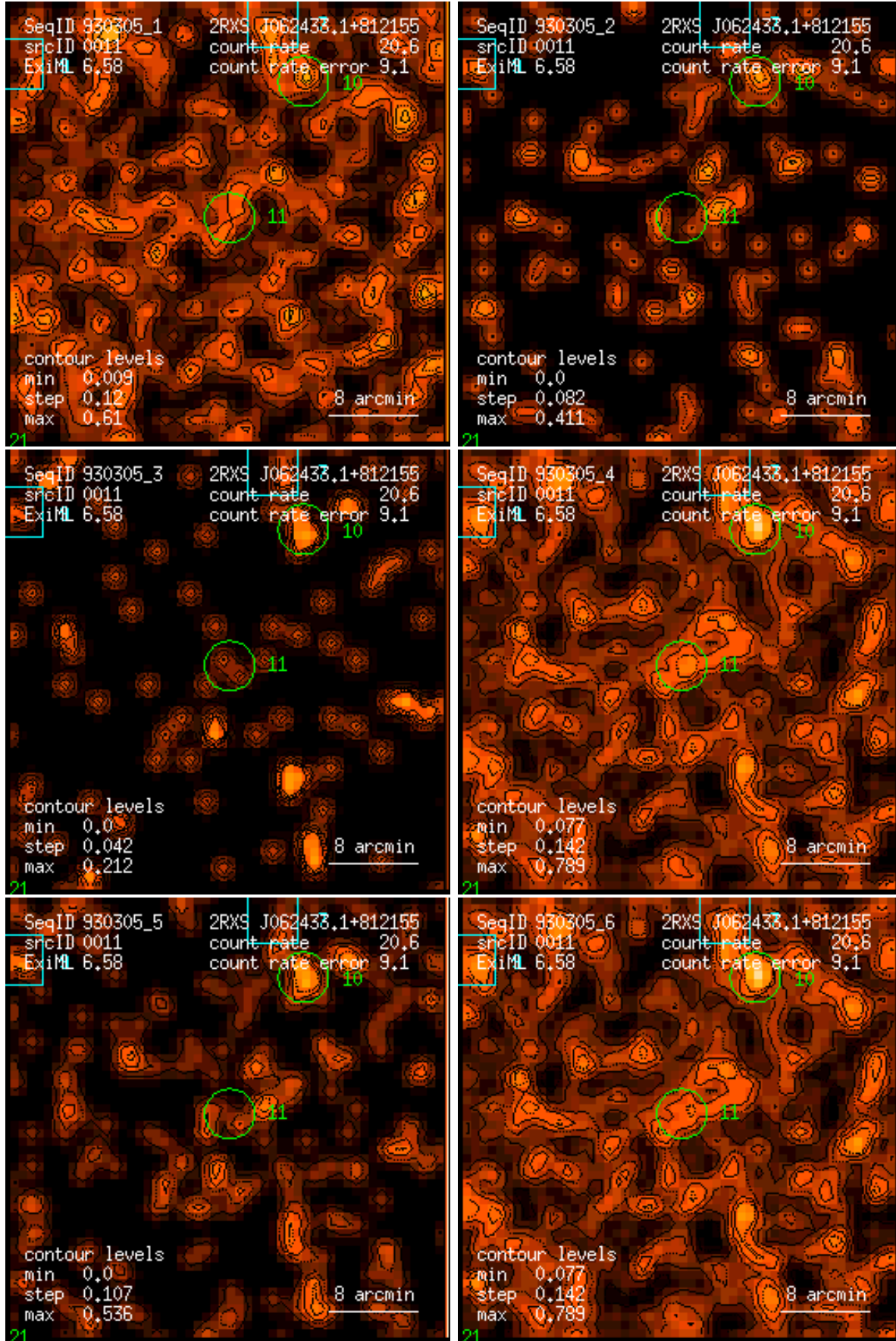
Figure 11: RASS 930305: detection 0011: band rate images, Gaussian filter: (1) PSPC channels 11 – 41, (2) 52 – 90, (3) 91 – 201, (4) 11 – 235, (5) 52 – 201, (6) 11 – 201. Broad band rates in counts/ks. Band rate contour levels in counts/ks/arcmin 2 .
