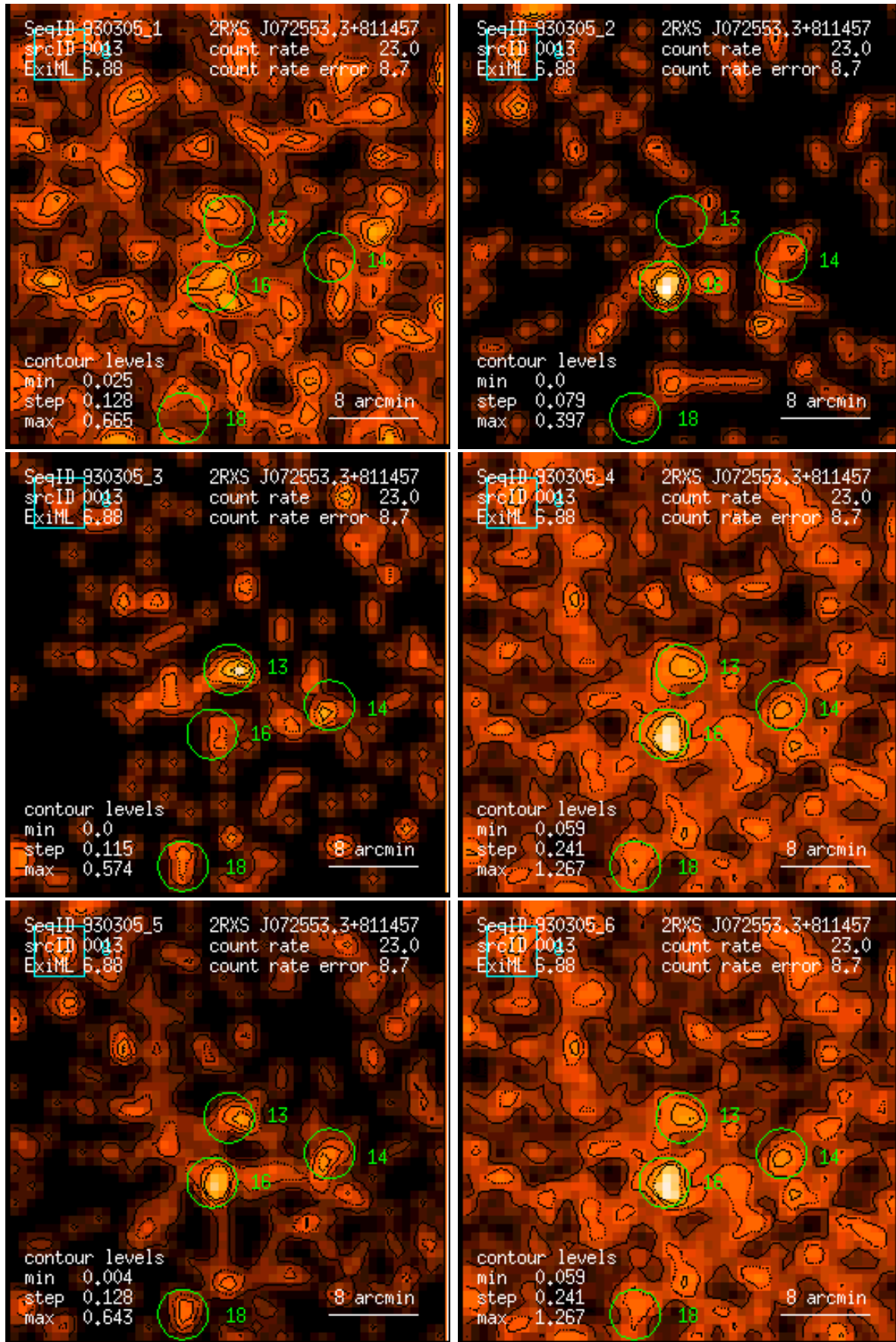
Figure 13: RASS 930305: detection 0013: band rate images, Gaussian filter: (1) PSPC channels 11 – 41, (2) 52 – 90, (3) 91 – 201, (4) 11 – 235, (5) 52 – 201, (6) 11 – 201. Broad band rates in counts/ks. Band rate contour levels in counts/ks/arcmin 2 .
