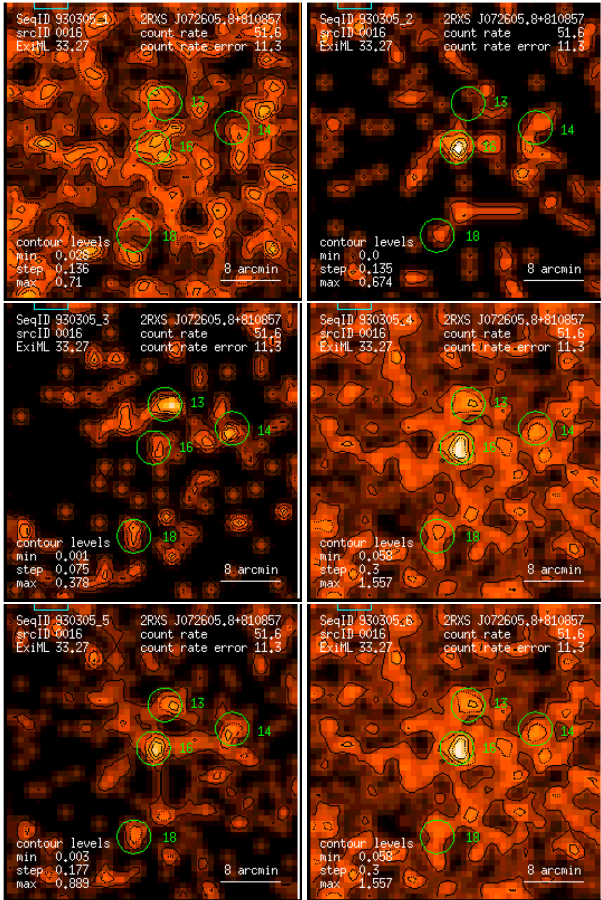
Figure 16: RASS 930305: detection 0016: band rate images, Gaussian filter: (1) PSPC channels 11 – 41, (2) 52 – 90, (3) 91 – 201, (4) 11 – 235, (5) 52 – 201, (6) 11 – 201. Broad band rates in counts/ks. Band rate contour levels in counts/ks/arcmin 2 .
