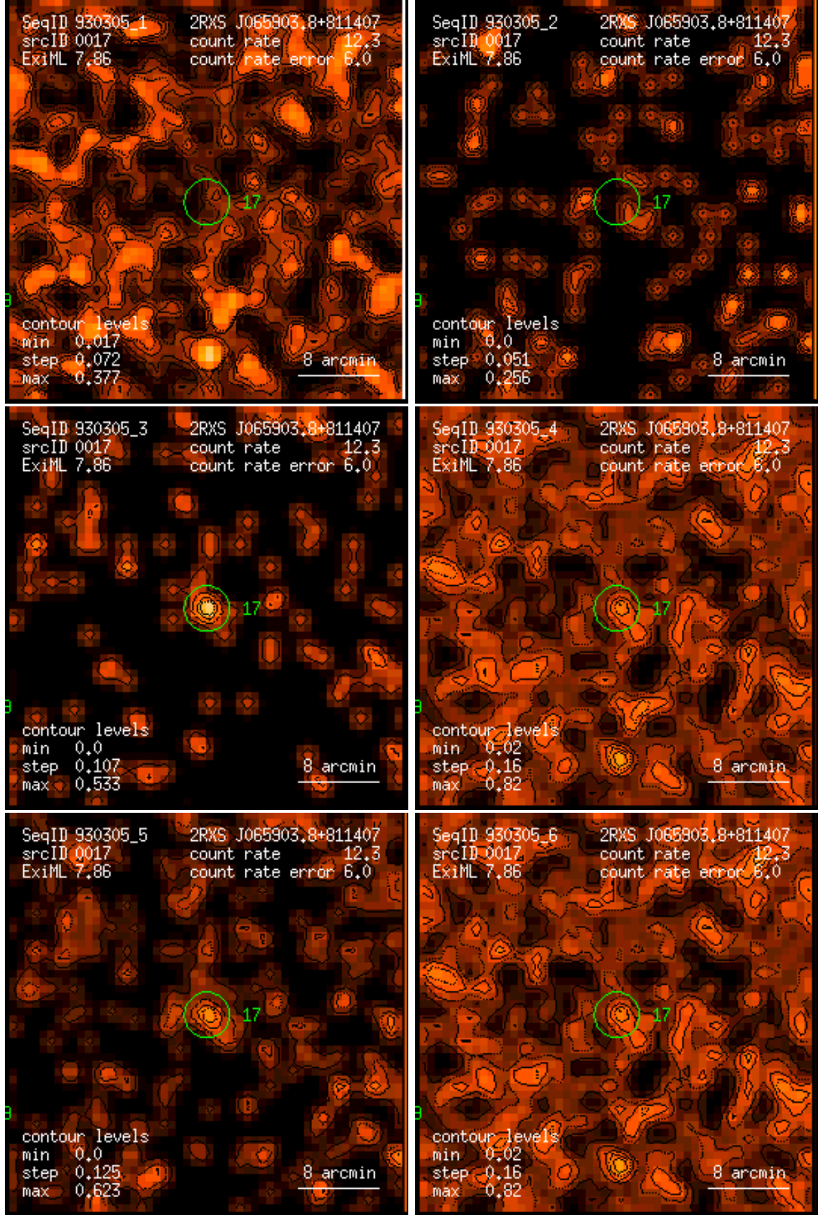
Figure 17: RASS 930305: detection 0017: band rate images, Gaussian filter: (1) PSPC channels 11 – 41, (2) 52 – 90, (3) 91 – 201, (4) 11 – 235, (5) 52 – 201, (6) 11 – 201. Broad band rates in counts/ks. Band rate contour levels in counts/ks/arcmin 2 .
