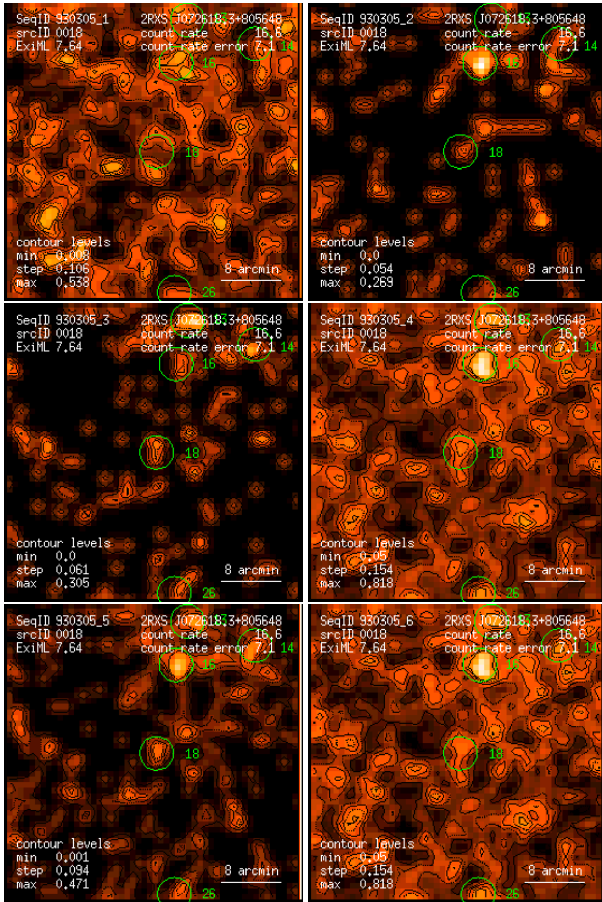
Figure 18: RASS 930305: detection 0018: band rate images, Gaussian filter: (1) PSPC channels 11 – 41, (2) 52 – 90, (3) 91 – 201, (4) 11 – 235, (5) 52 – 201, (6) 11 – 201. Broad band rates in counts/ks. Band rate contour levels in counts/ks/arcmin 2 .
