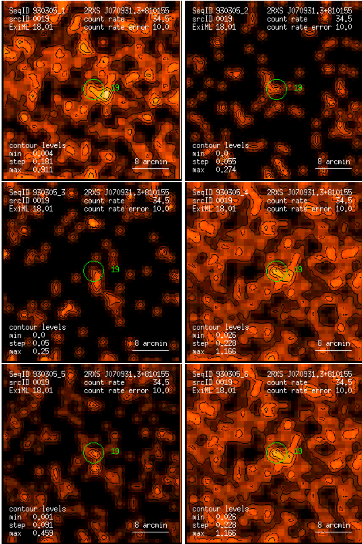
Figure 19: RASS 930305: detection 0019: band rate images, Gaussian filter: (1) PSPC channels 11 – 41, (2) 52 – 90, (3) 91 – 201, (4) 11 – 235, (5) 52 – 201, (6) 11 – 201. Broad band rates in counts/ks. Band rate contour levels in counts/ks/arcmin 2 .
