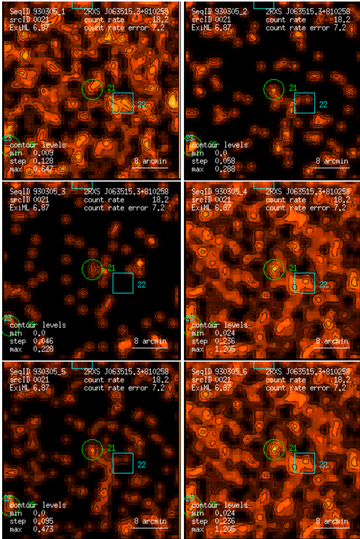
Figure 21: RASS 930305: detection 0021: band rate images, Gaussian filter: (1) PSPC channels 11 – 41, (2) 52 – 90, (3) 91 – 201, (4) 11 – 235, (5) 52 – 201, (6) 11 – 201. Broad band rates in counts/ks. Band rate contour levels in counts/ks/arcmin 2 .
