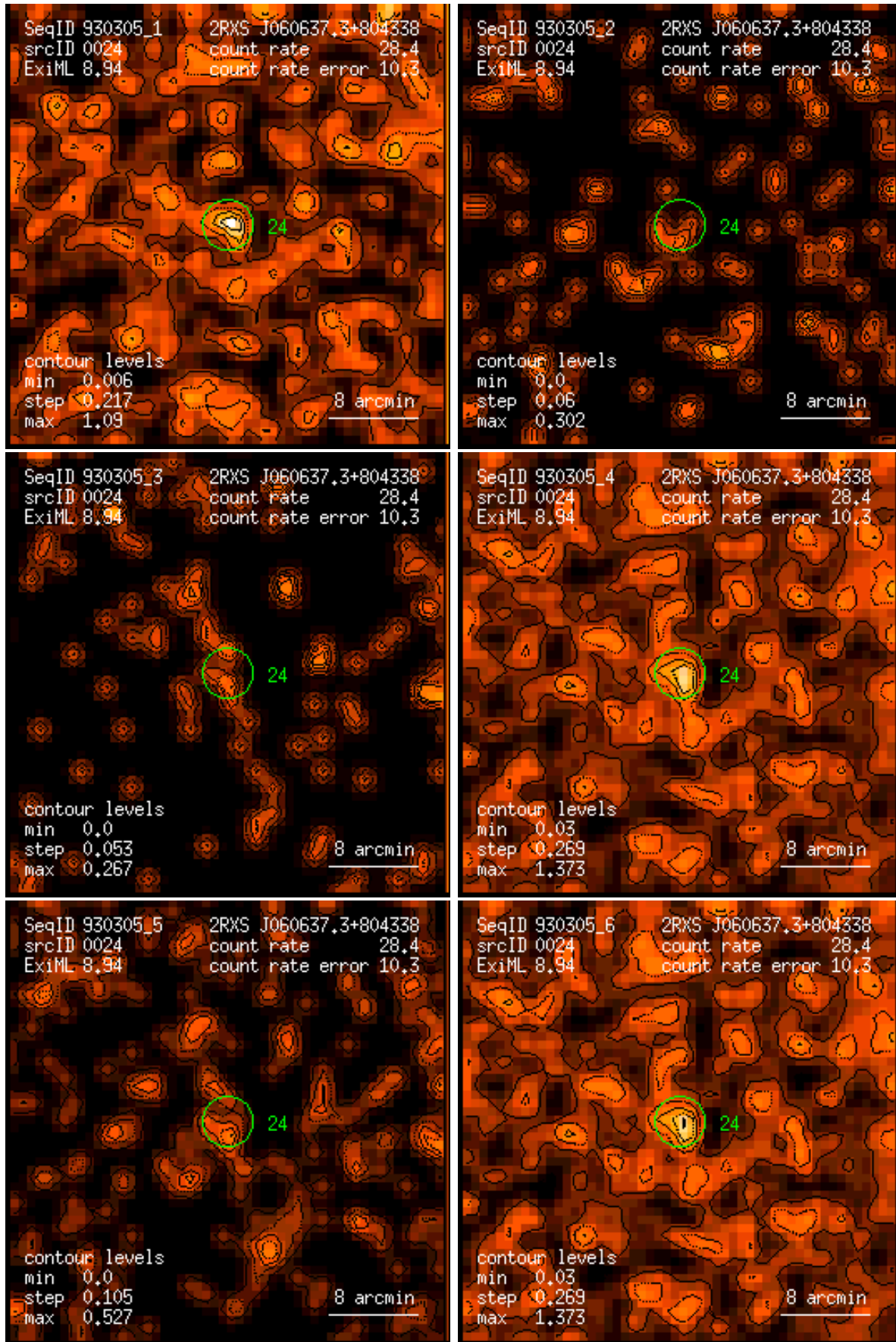
Figure 24: RASS 930305: detection 0024: band rate images, Gaussian filter: (1) PSPC channels 11 – 41, (2) 52 – 90, (3) 91 – 201, (4) 11 – 235, (5) 52 – 201, (6) 11 – 201. Broad band rates in counts/ks. Band rate contour levels in counts/ks/arcmin 2 .
