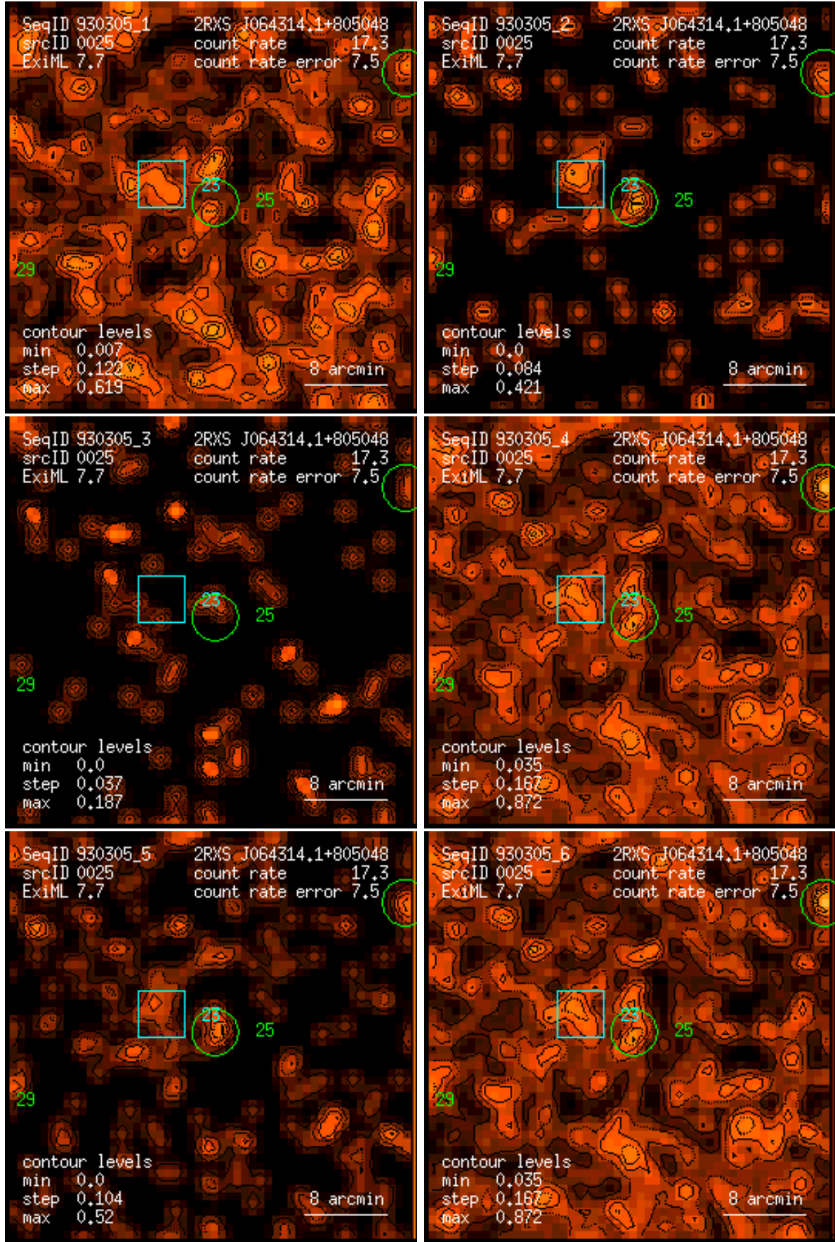
Figure 25: RASS 930305: detection 0025: band rate images, Gaussian filter: (1) PSPC channels 11 – 41, (2) 52 – 90, (3) 91 – 201, (4) 11 – 235, (5) 52 – 201, (6) 11 – 201. Broad band rates in counts/ks. Band rate contour levels in counts/ks/arcmin 2 .
