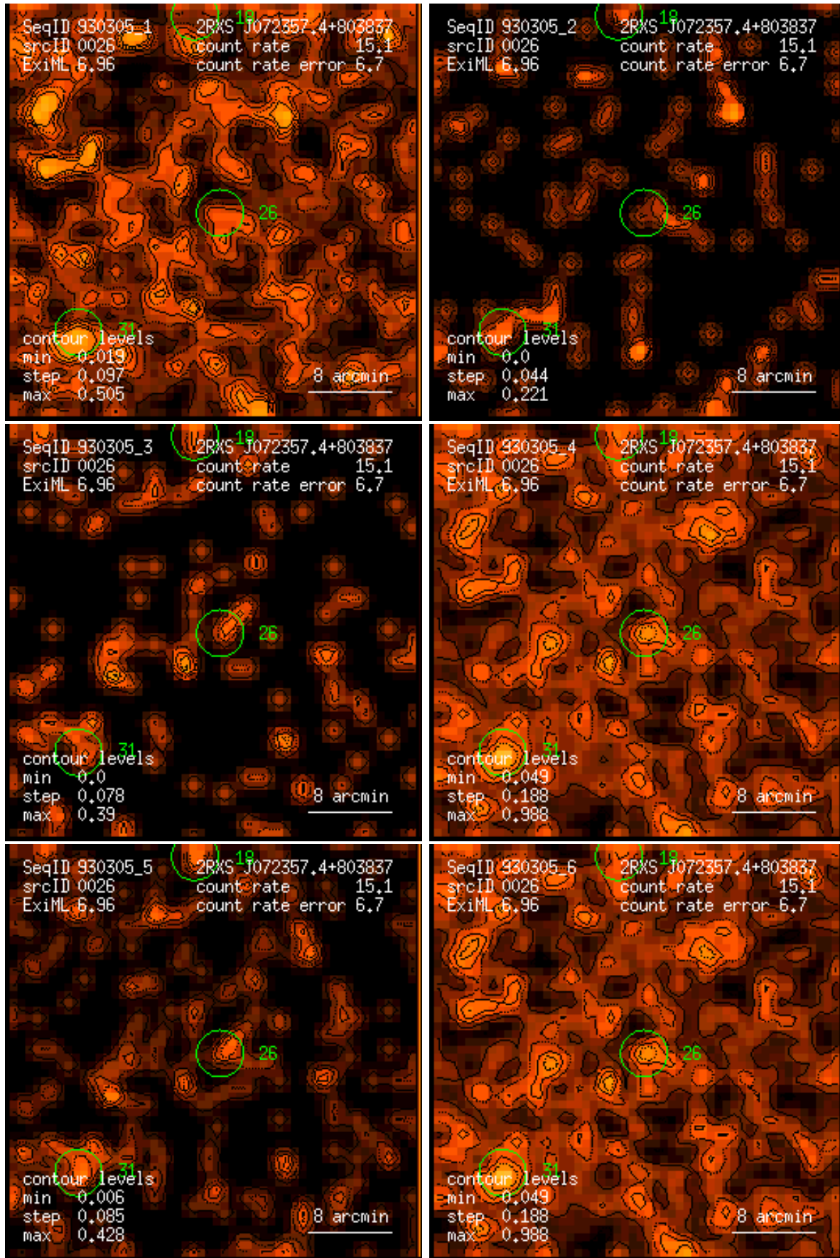
Figure 26: RASS 930305: detection 0026: band rate images, Gaussian filter: (1) PSPC channels 11 – 41, (2) 52 – 90, (3) 91 – 201, (4) 11 – 235, (5) 52 – 201, (6) 11 – 201. Broad band rates in counts/ks. Band rate contour levels in counts/ks/arcmin 2 .
