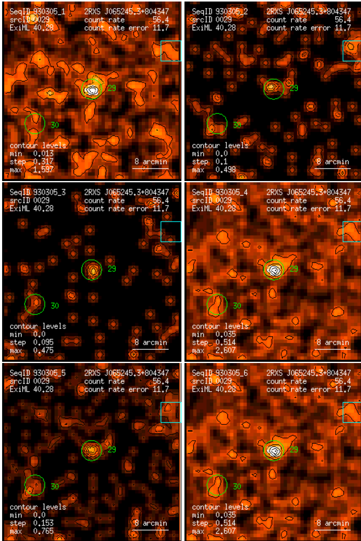
Figure 29: RASS 930305: detection 0029: band rate images, Gaussian filter: (1) PSPC channels 11 – 41, (2) 52 – 90, (3) 91 – 201, (4) 11 – 235, (5) 52 – 201, (6) 11 – 201. Broad band rates in counts/ks. Band rate contour levels in counts/ks/arcmin 2 .
