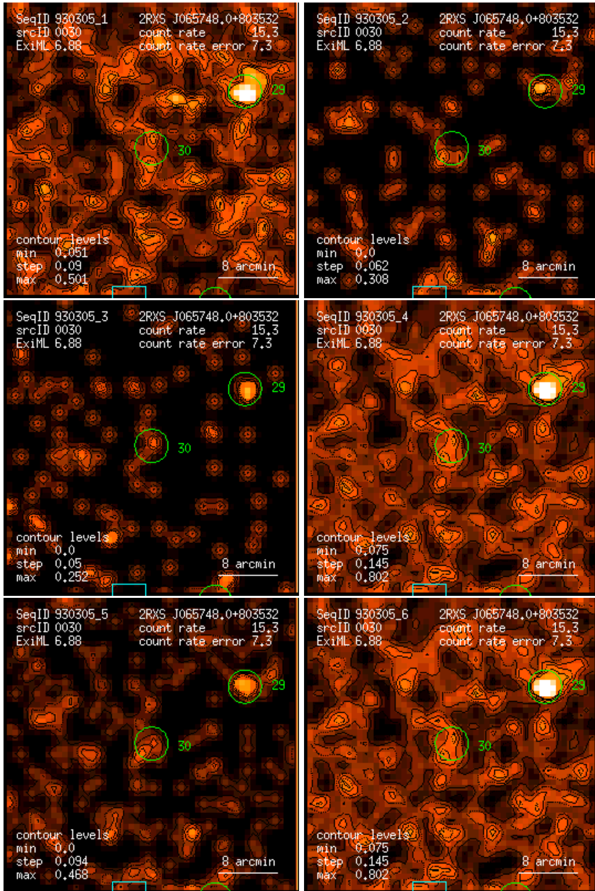
Figure 30: RASS 930305: detection 0030: band rate images, Gaussian filter: (1) PSPC channels 11 – 41, (2) 52 – 90, (3) 91 – 201, (4) 11 – 235, (5) 52 – 201, (6) 11 – 201. Broad band rates in counts/ks. Band rate contour levels in counts/ks/arcmin 2 .
