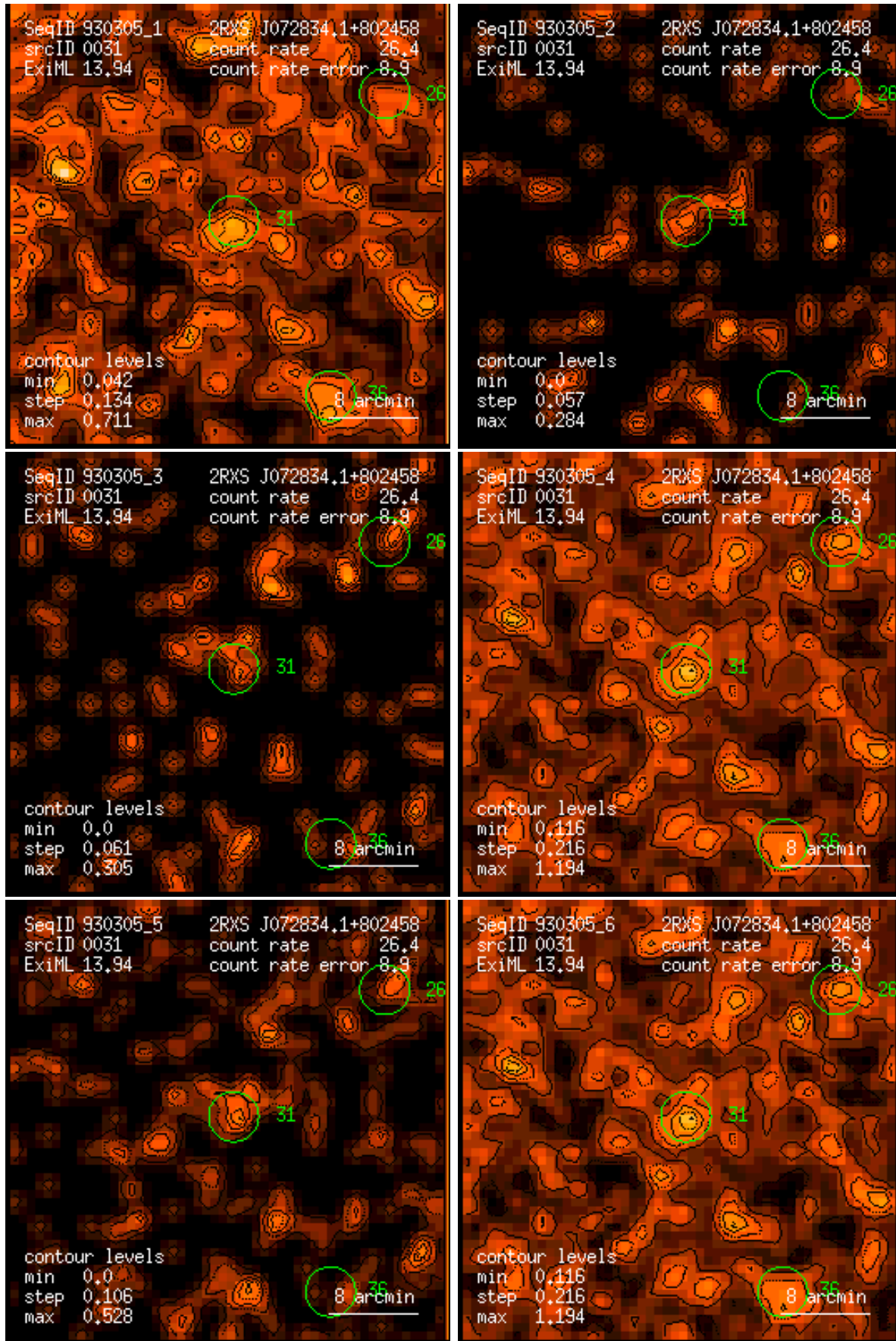
Figure 31: RASS 930305: detection 0031: band rate images, Gaussian filter: (1) PSPC channels 11 – 41, (2) 52 – 90, (3) 91 – 201, (4) 11 – 235, (5) 52 – 201, (6) 11 – 201. Broad band rates in counts/ks. Band rate contour levels in counts/ks/arcmin 2 .
