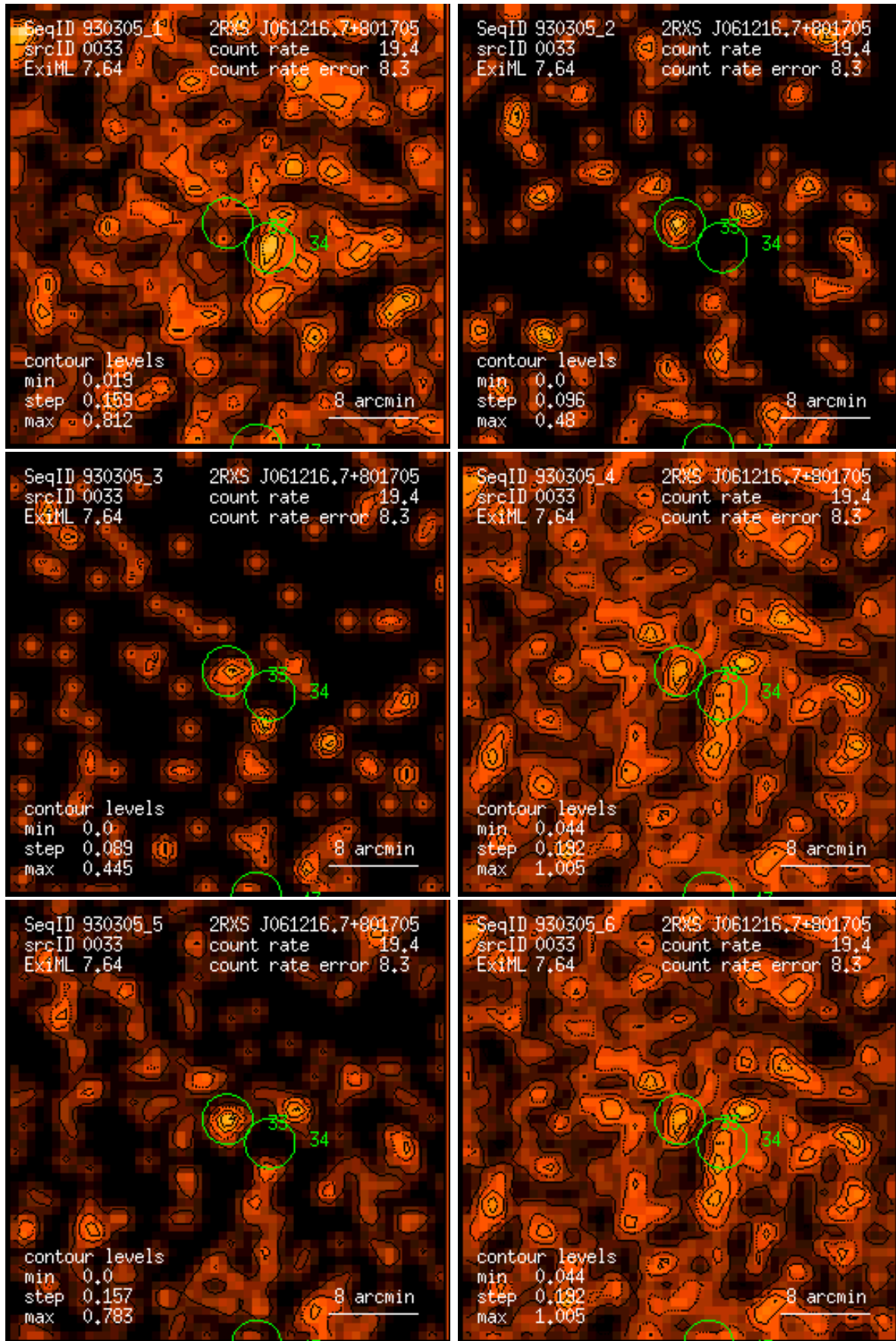
Figure 33: RASS 930305: detection 0033: band rate images, Gaussian filter: (1) PSPC channels 11 – 41, (2) 52 – 90, (3) 91 – 201, (4) 11 – 235, (5) 52 – 201, (6) 11 – 201. Broad band rates in counts/ks. Band rate contour levels in counts/ks/arcmin 2 .
