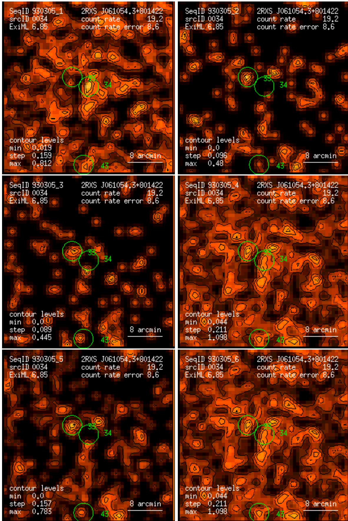
Figure 34: RASS 930305: detection 0034: band rate images, Gaussian filter: (1) PSPC channels 11 – 41, (2) 52 – 90, (3) 91 – 201, (4) 11 – 235, (5) 52 – 201, (6) 11 – 201. Broad band rates in counts/ks. Band rate contour levels in counts/ks/arcmin 2 .
